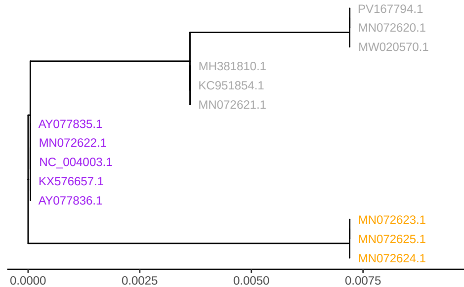
GTPV gene LSDV061
