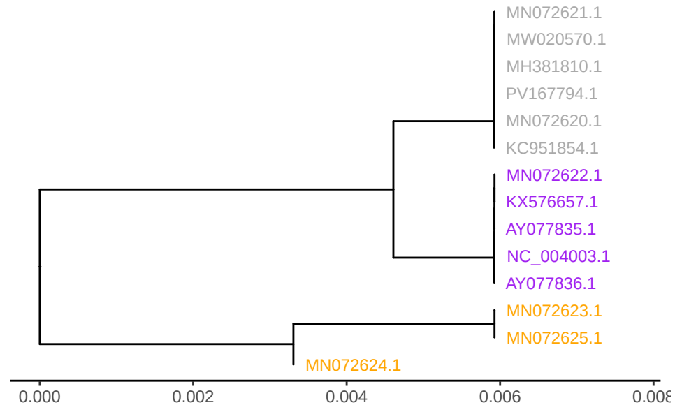
GTPV gene LSDV063
