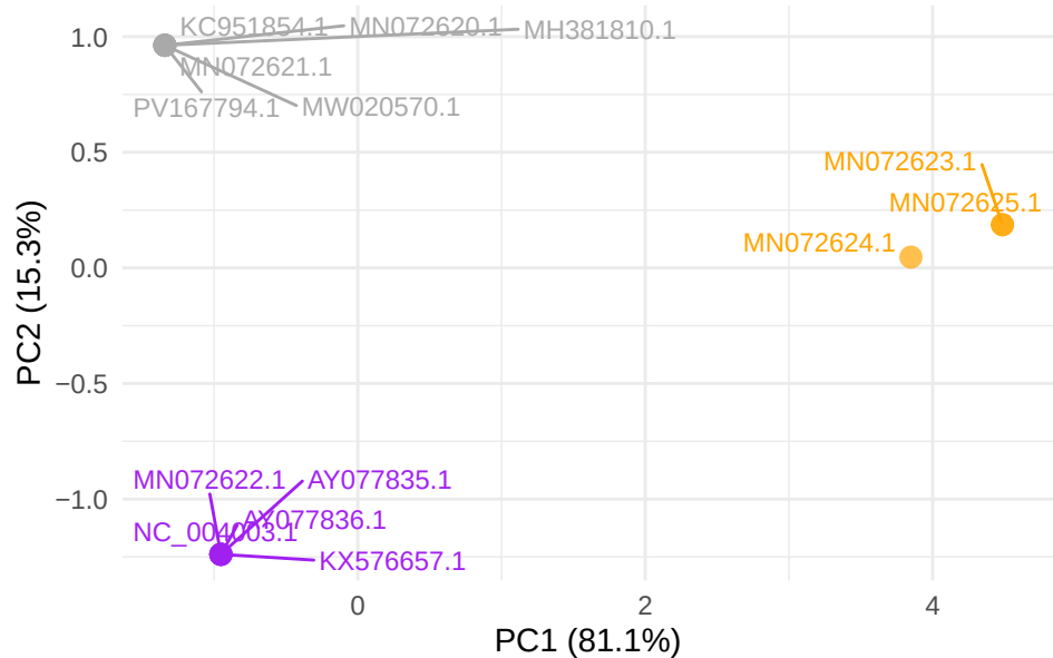
GTPV gene LSDV063
