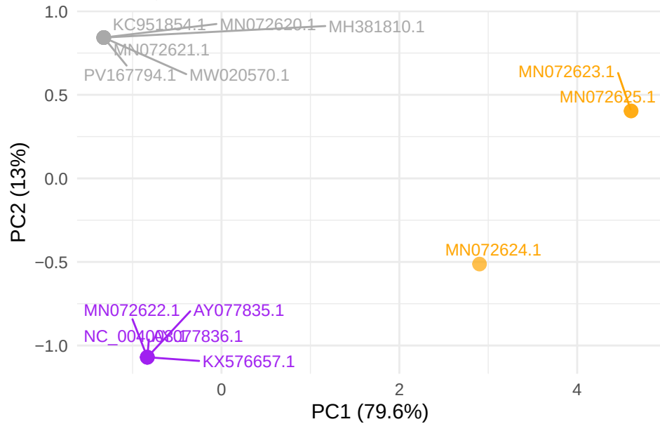
GTPV gene LSDV073
