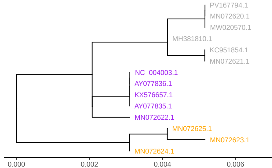
GTPV gene LSDV074
