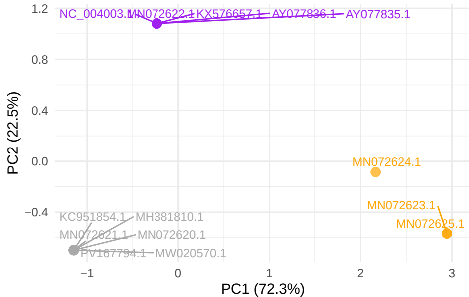
GTPV gene LSDV077
