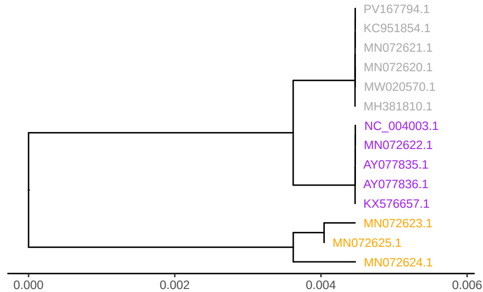
GTPV gene LSDV083
