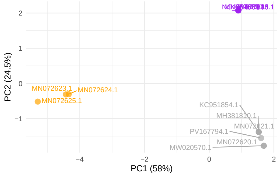
GTPV gene LSDV090
