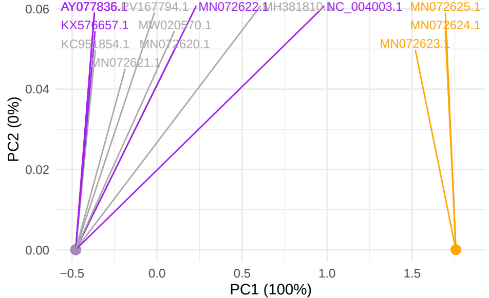
GTPV gene LSDV093
