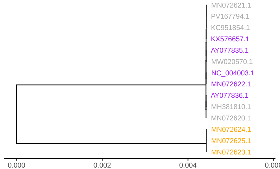
GTPV gene LSDV093
