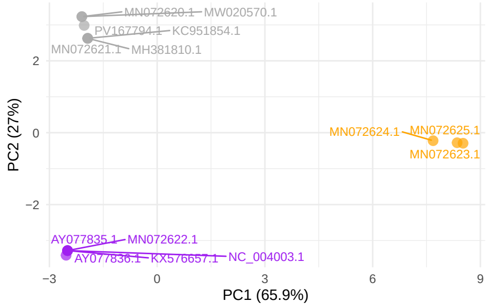
GTPV gene LSDV101
