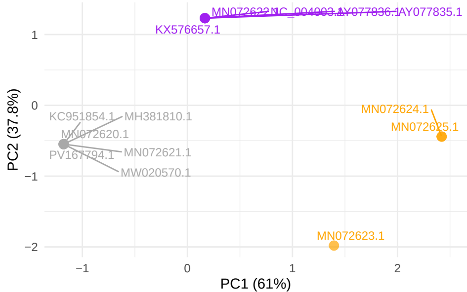
GTPV gene LSDV105
