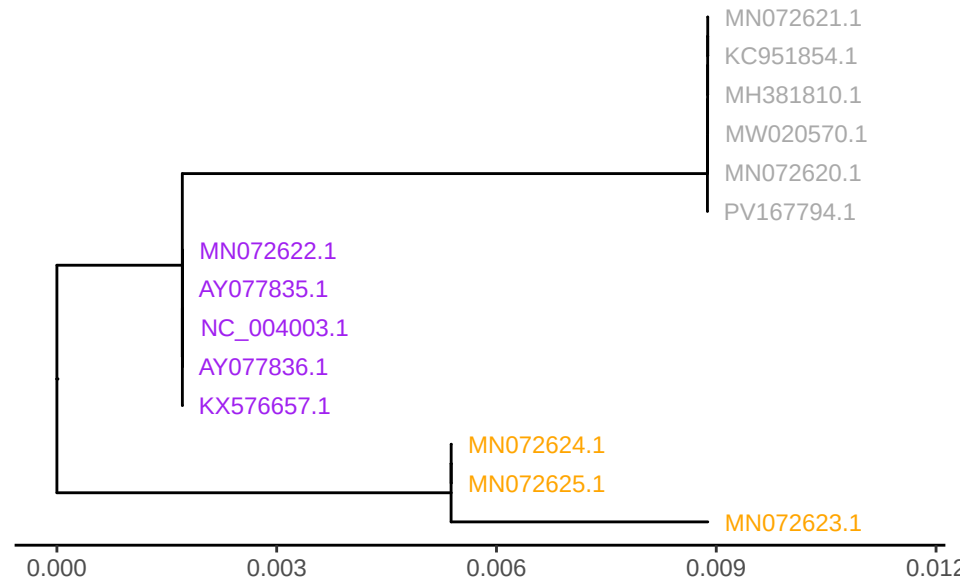
GTPV gene LSDV105
