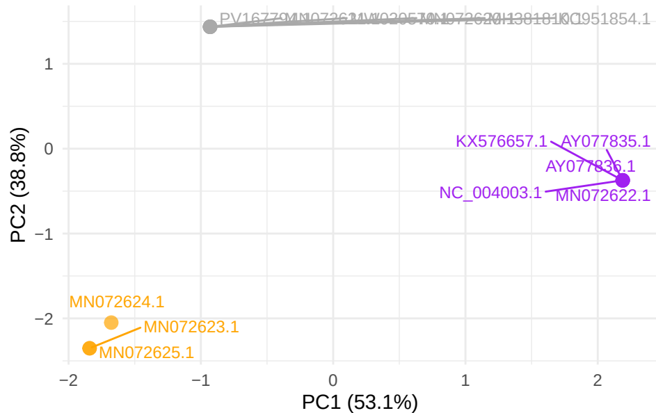
GTPV gene LSDV119
