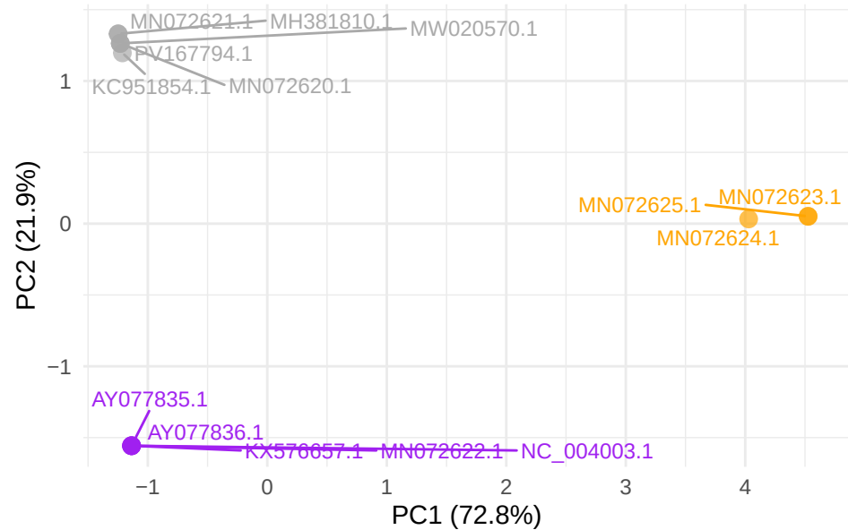
GTPV gene LSDV122
