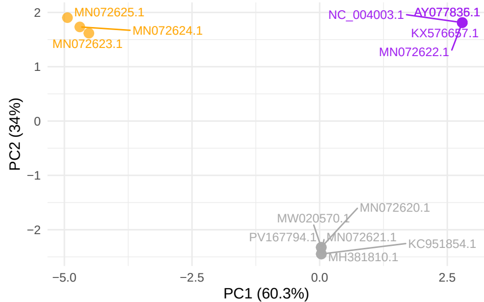
GTPV gene LSDV128
