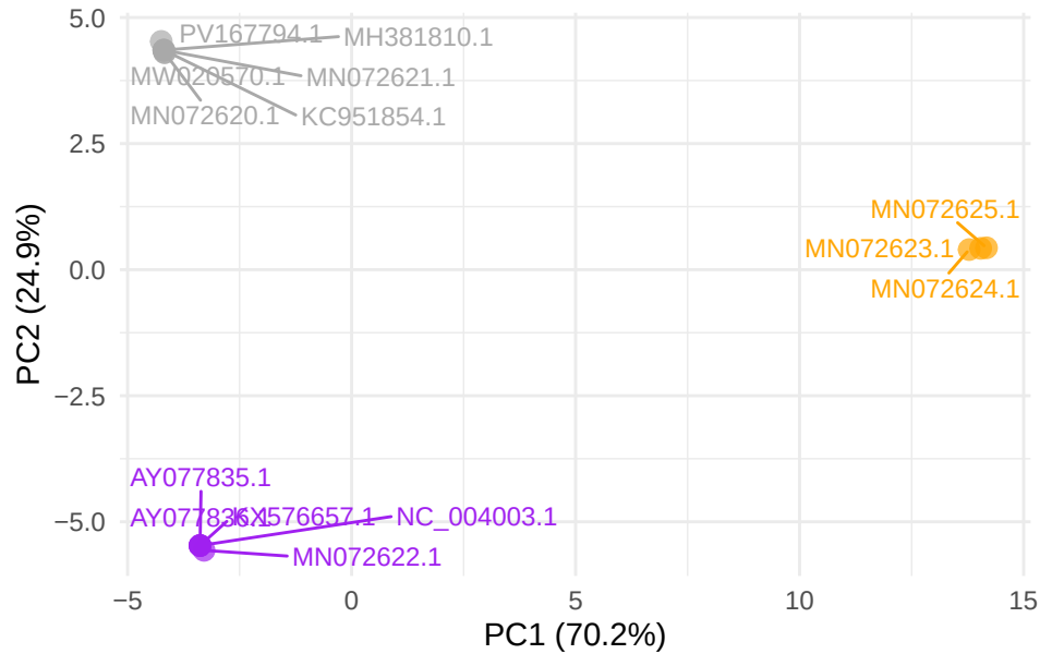
GTPV gene LSDV134
