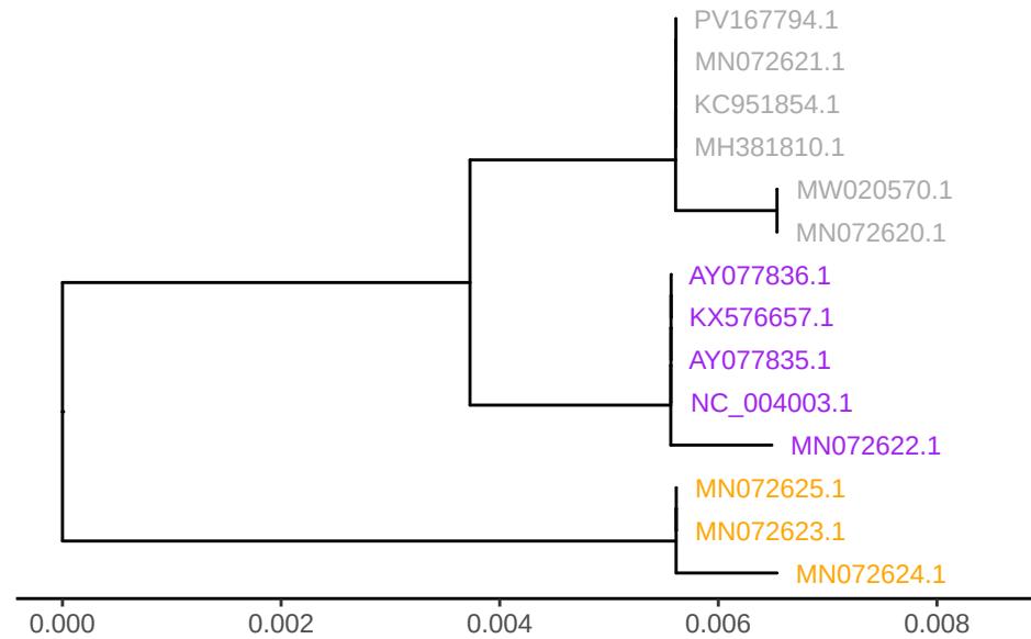
GTPV gene LSDV135
