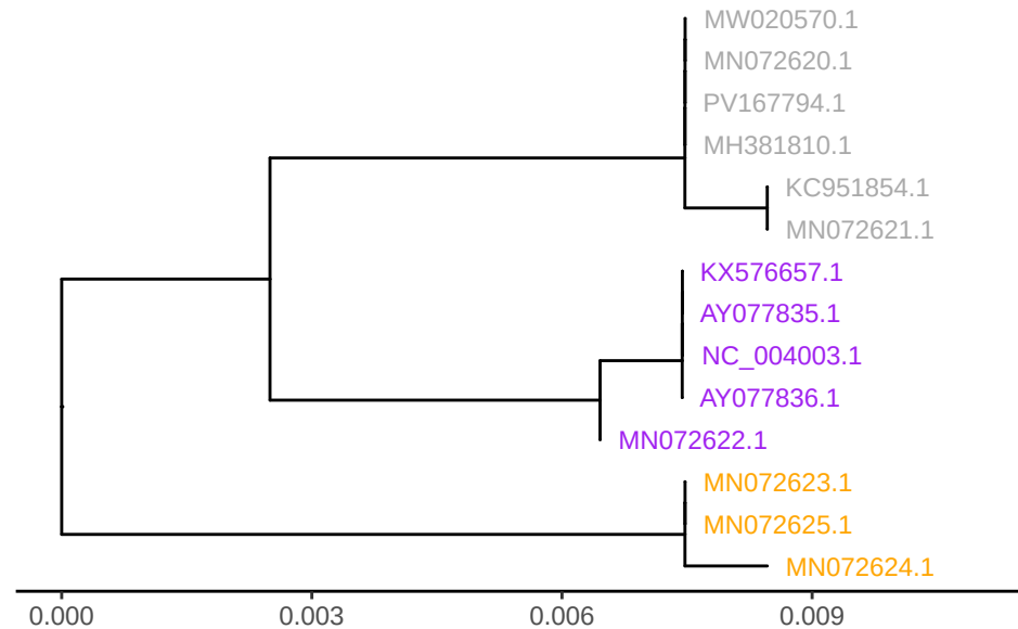
GTPV gene LSDV149
