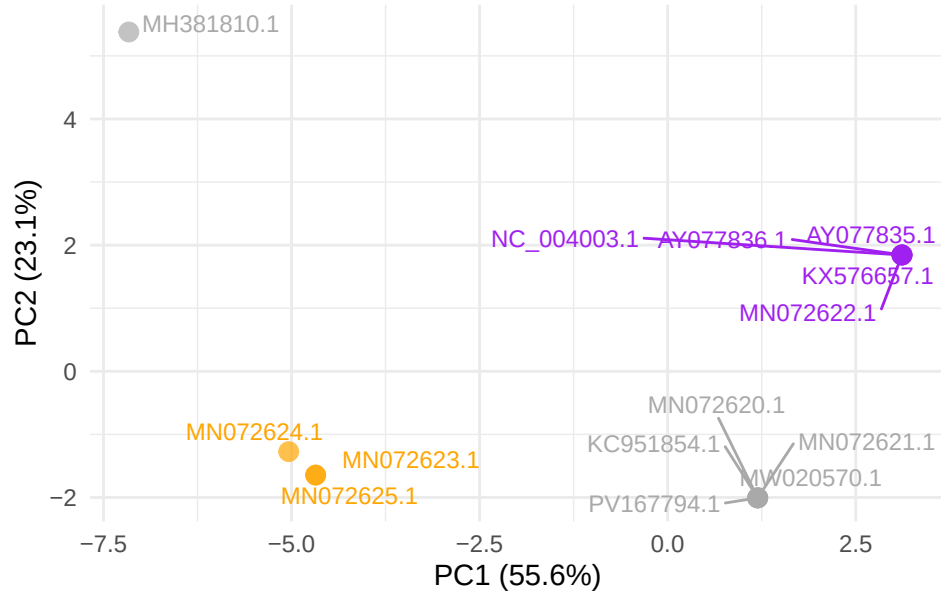
GTPV gene LSDV155
