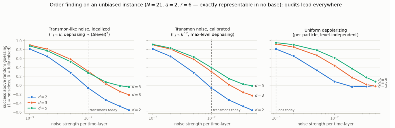
FIG. 3. Unbiased-instance noise sweep ( N = 21 , a = 2 , r = 6 ), exact density-matrix evolution, uniform cost model (native entangler). Floor-corrected signal vs noise strength for the idealized ladder, calibrated ladder, and per-particle depolarizing channels. The best qudit leads the qubit at every strength under all three models; the single exception to a uniform qudit lead is the deepest depolarizing point ( s = 0.05 ), where the qutrit alone dips marginally below the qubit with all signals within 0.09 of zero.
