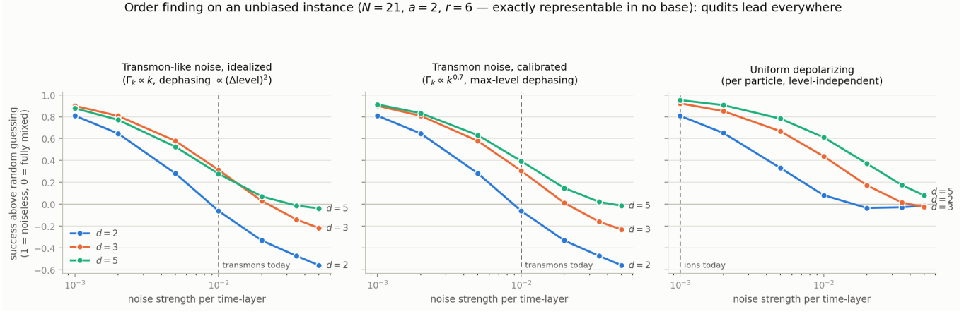
FIG. 3. Unbiased-instance noise sweep ( N = 21, a = 2, r = 6 ), exact density-matrix evolution, uniform cost model (native entangler). Floor-corrected signal vs noise strength for the idealized ladder, calibrated ladder, and per-particle depolarizing channels. The best qudit leads the qubit at every strength under all three models; the single exception to a uniform qudit lead is the deepest depolarizing point ( s = 0.05 ), where the qutrit alone dips marginally below the qubit with all signals within 0.08 of zero.
