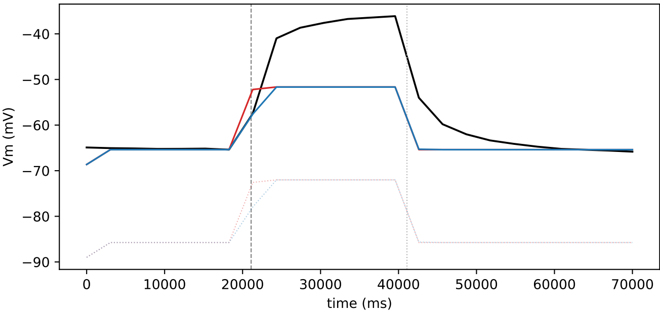
sweep 5 | current 150 nA LS: centered RMSE 7.63, end \Delta -15.5 | NSGA2: centered RMSE 7.55, end \Delta -15.5
