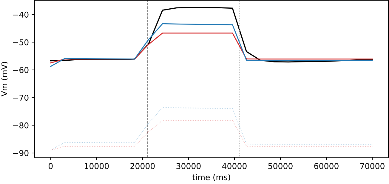
sweep 6 | current 175 nA LS: centered RMSE 4.56, end \Delta -9.0 | NSGA2: centered RMSE 3.05, end \Delta -6.0
