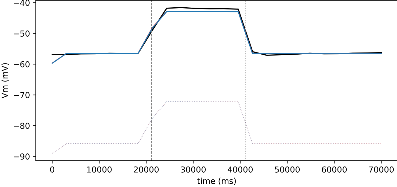
sweep 5 | current 150 nA LS: centered RMSE 3.55, end \Delta -6.5 | NSGA2: centered RMSE 3.55, end \Delta -6.6
