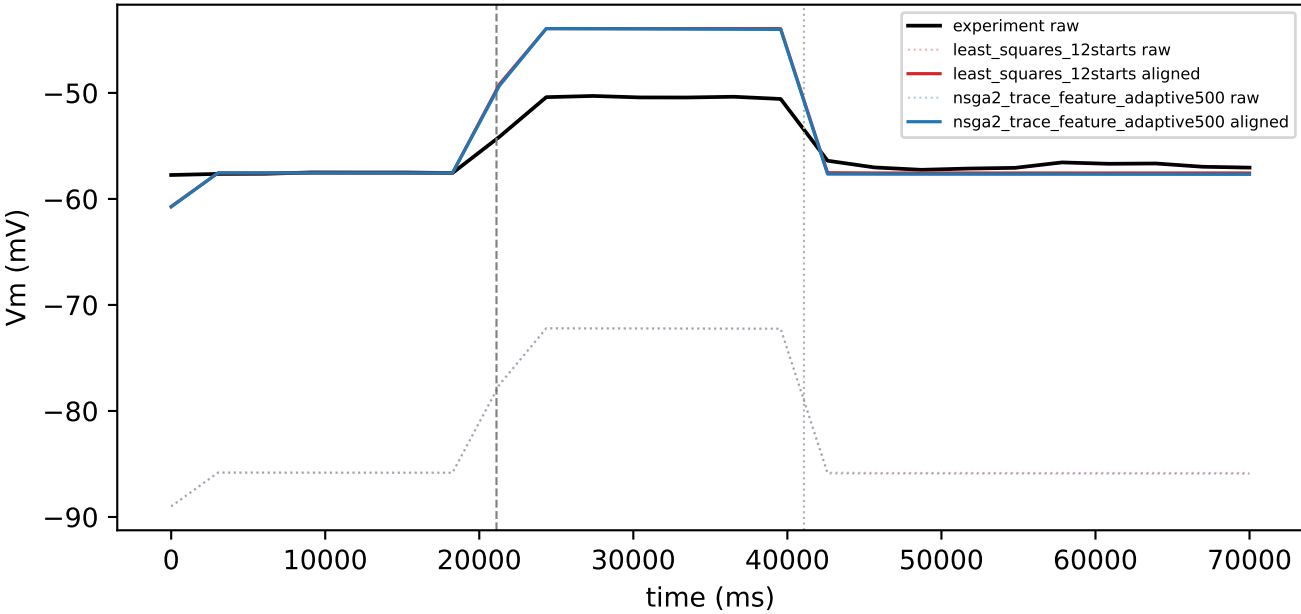
sweep 1 | current 50 nA LS: centered RMSE 3.48, end \Delta 6.6 | NSGA2: centered RMSE 3.47, end \Delta 6.6
