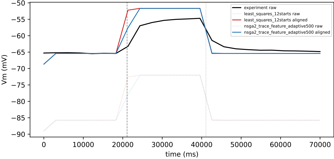
sweep 1 | current 50 nA LS: centered RMSE 3.24, end \Delta 3.0 | NSGA2: centered RMSE 2.59, end \Delta 3.0
