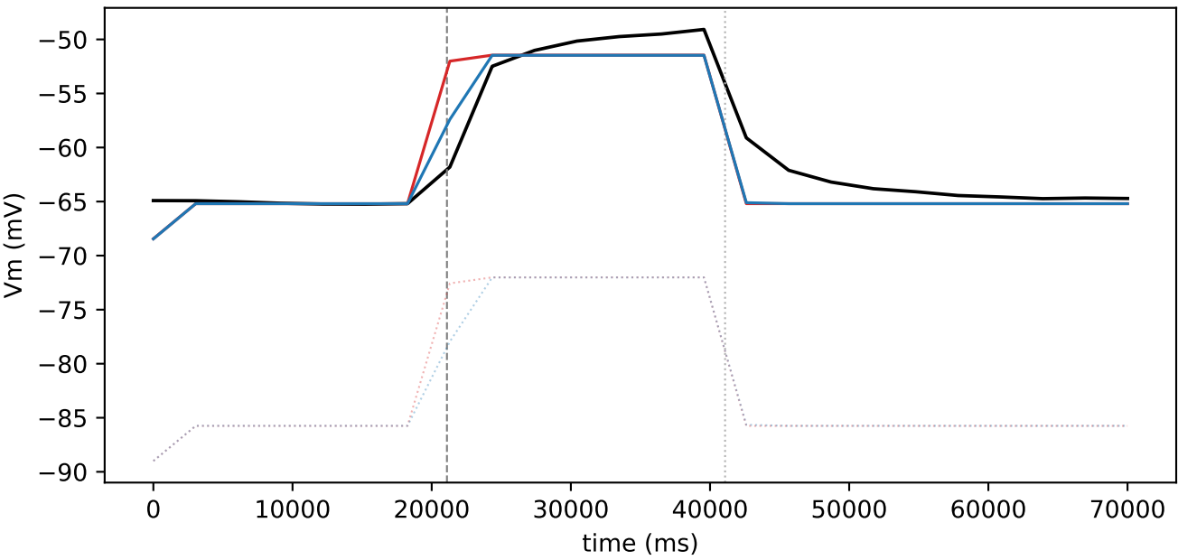
sweep 2 | current 75 nA LS: centered RMSE 2.73, end \Delta -2.4 | NSGA2: centered RMSE 2.06, end \Delta -2.4
