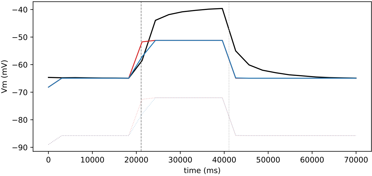
sweep 4 | current 125 nA LS: centered RMSE 5.85, end \Delta -11.6 | NSGA2: centered RMSE 5.69, end \Delta -11.6
