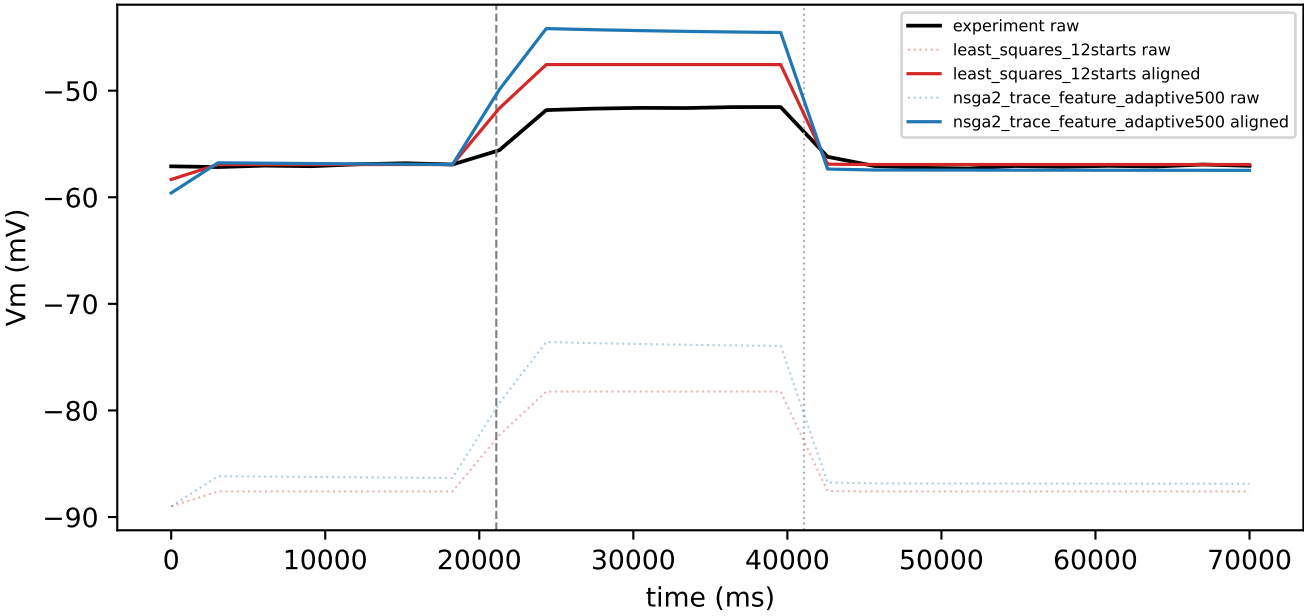
sweep 1 | current 50 nA LS: centered RMSE 2.22, end \Delta 4.0 | NSGA2: centered RMSE 3.86, end \Delta 7.0
