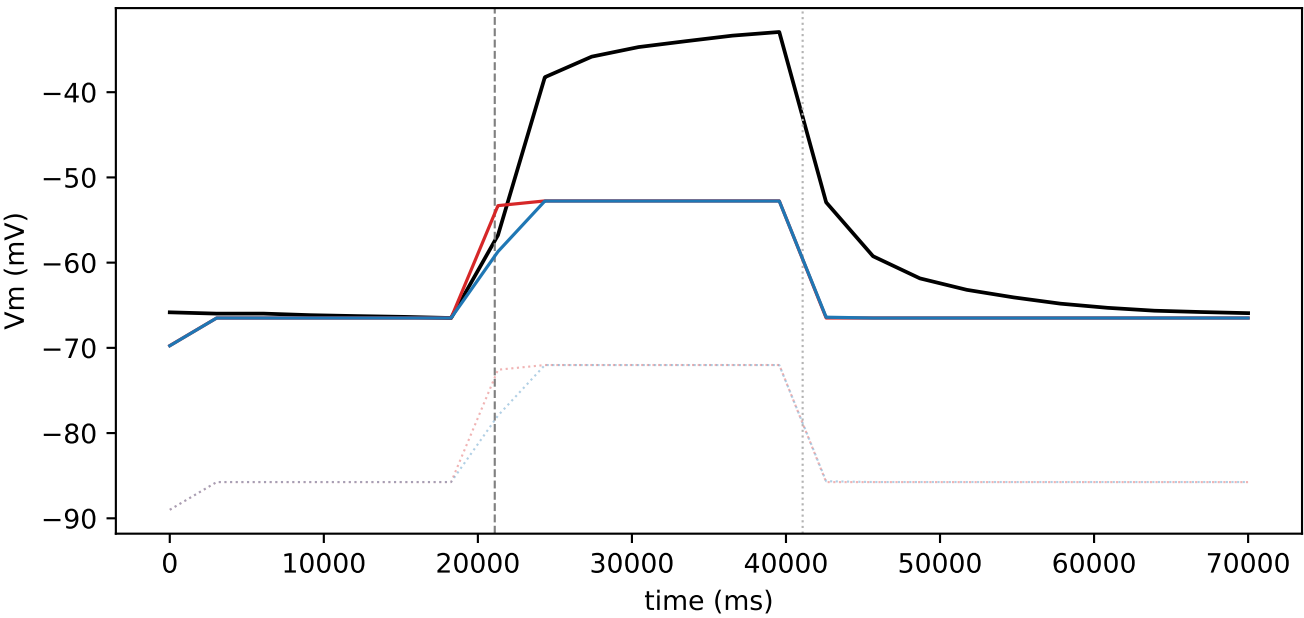
sweep 6 | current 175 nA LS: centered RMSE 9.69, end \Delta -19.8 | NSGA2: centered RMSE 9.67, end \Delta -19.8
