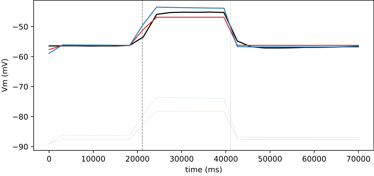
sweep 5 | current 150 nA LS: centered RMSE 3.39, end \Delta -6.7 | NSGA2: centered RMSE 1.98, end \Delta -3.6
