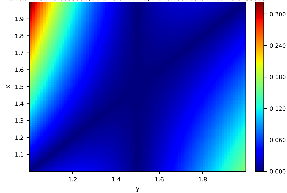
Error, RMSE=0.0695594, MAE=0.0444471, ME=0.0397134, MRED=0.0435025
