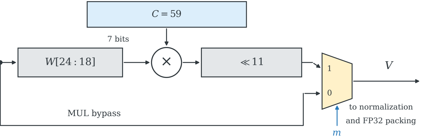
(c) DIV scaling and mode selection
