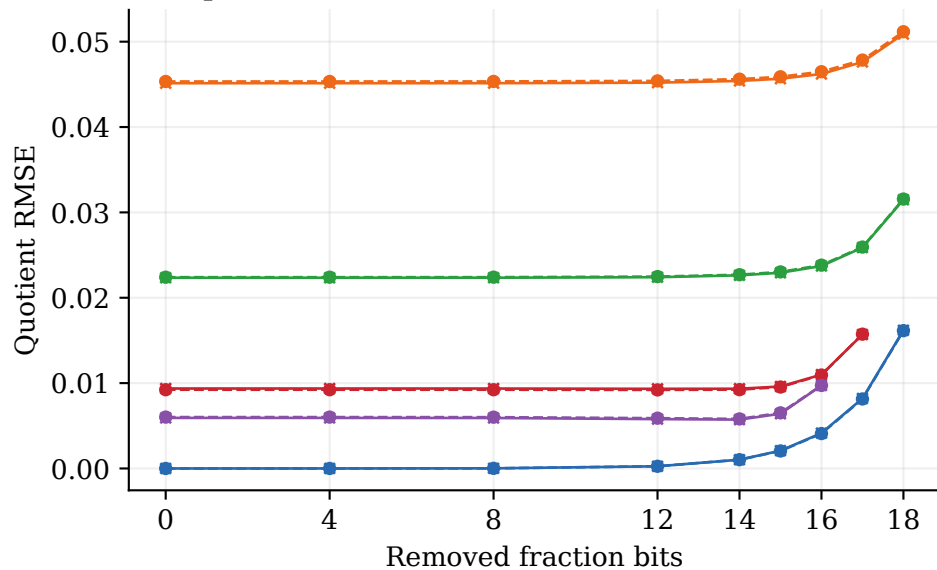
Paper (dashed) and reconstructed RTL (solid)
