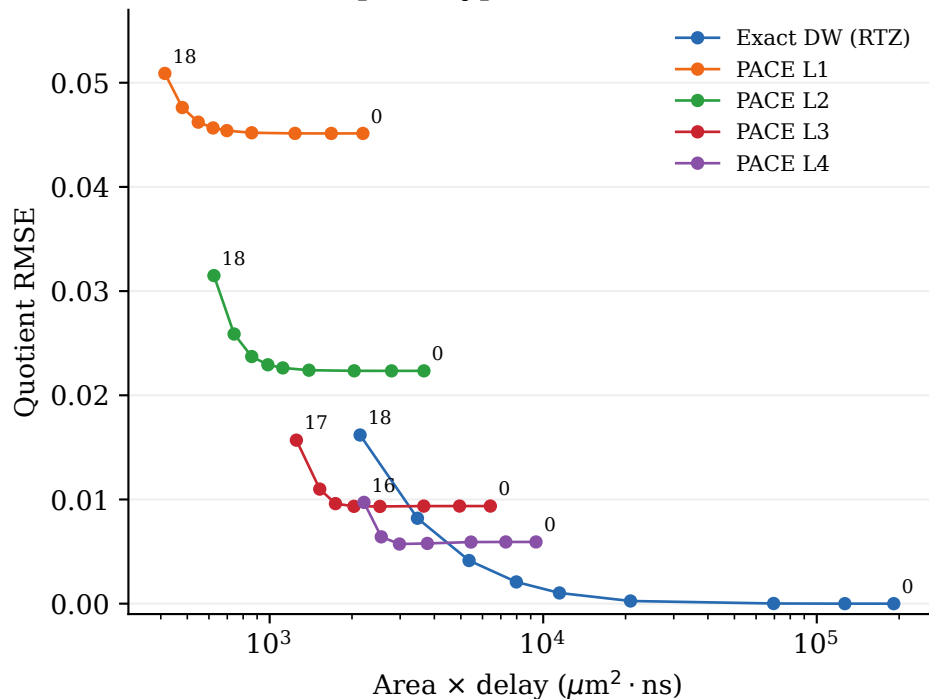
Whole-datapath hypothesis: TSMC65, 10 ns
