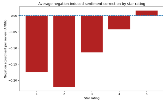
Figure 16: Average Negation-Induced Sentiment Correction by Star Rating in Python
