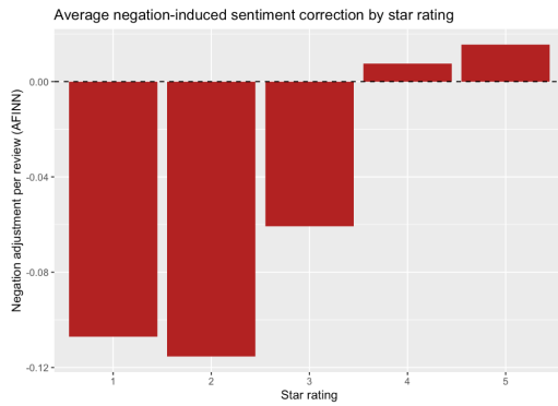
Figure 15: Average Negation-Induced Sentiment Correction by Star Rating in R
