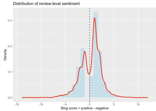
Figure 5: Distribution of Review-Level Bing Sentiment Scores in R
