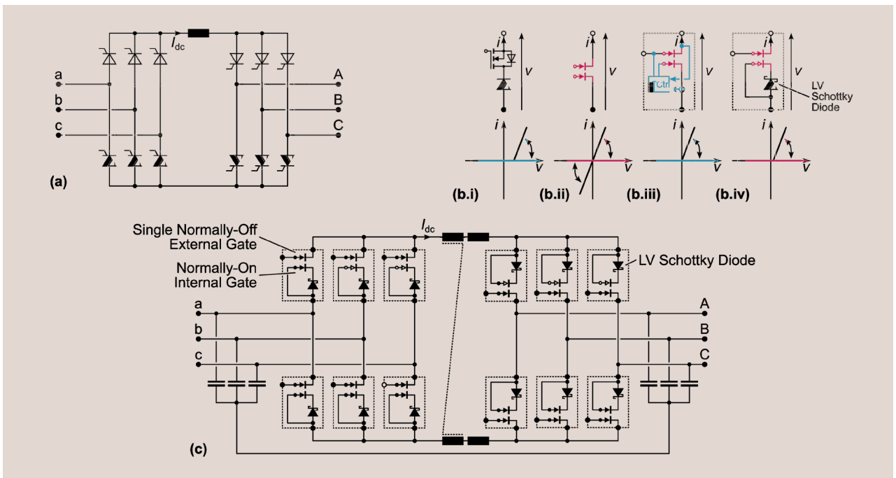
FIG 11 (a) Motor drive based on line-commutated inverters (LCI). (b) Realization of the minimum required functionality (bipolar voltage blocking but only unidirectional current conduction) for ac-ac current-source converters (CSCs) without the drawback of (b.i) a high-voltage series diode by using (b.ii) MBDSs and, to reduce complexity, (b.iii) advanced self-switching gate drives [23] or (b.iv) a cascode configuration of a MBDS and a low-voltage Schottky diode (self-reverse-blocking MBDS, SRB-MBDS) [22]; (c) SRB-MBDS-based ac-ac CSC.
