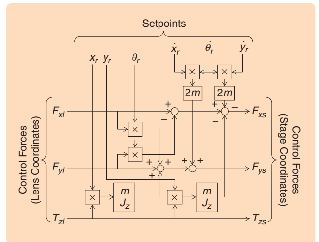
FIGURE 29 Gain scheduling of the horizontal control forces. Forces in the x and y directions are corrected by additional forces proportional to the torque T_z . In addition, the scheme shows a Coriolis correction as well as a correction for a nominal value of \theta not equaling zero.
