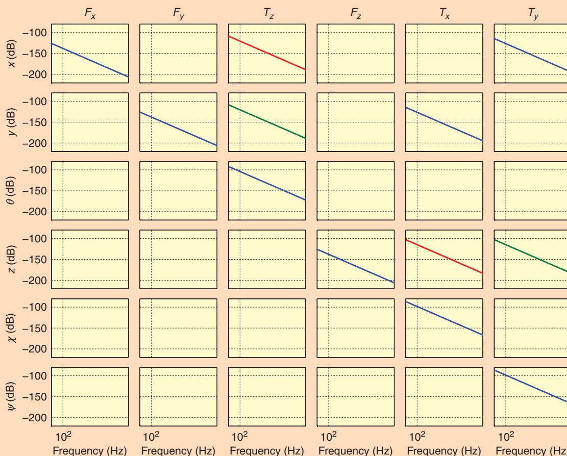
FIGURE 30 Stage transfer function. Each column represents the responses in all degrees of freedom to a force or torque in the direction indicated above the column. The response depends on the position of the stage in the horizontal plane. The blue lines show the response at (x, y) = (0, 0) , the green lines at (x, y) = (0.15, 0) , and the red lines at (x, y) = (0, 0.15) . All off-diagonal terms vanish when applying gain scheduling, leaving a perfectly decoupled 6 \times 6 system allowing six single-input, single-output controllers to be used.
