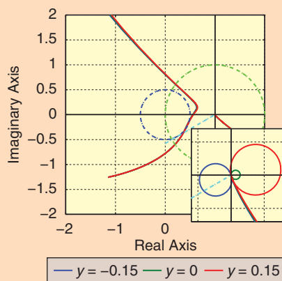
FIGURE 33 Nyquist plot of the z -controller open loop for three y positions. The inset shows the magnified behavior around the origin. This graph further elucidates the position dependence of the dynamical behavior.
