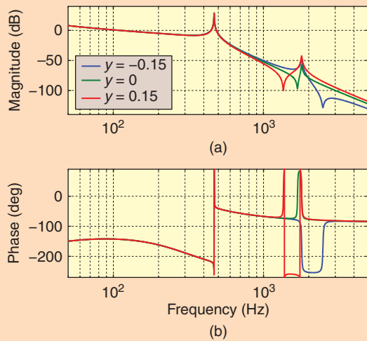
FIGURE 32 Bode plot of the z -controller open loop for three y positions. The resonances in all three cases coincide with the 500-Hz z mode and 1800-Hz \chi mode. Because the \chi mode is observed differently in the z measurement for different y positions, the anti-resonance frequency and phase behavior in the transfer function change. This change is not a problem because the magnitude of the 1800-Hz resonance is small.
