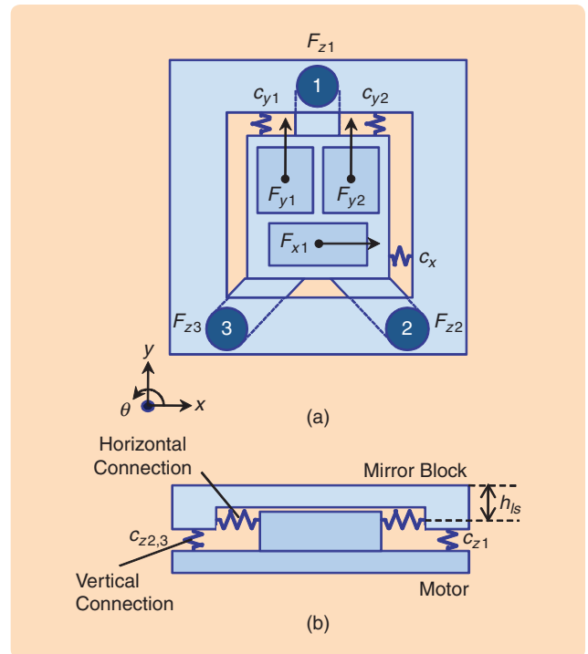
FIGURE 26 Stage layout with motor connection stiffness. The motor block, which is driven by the long-stroke motor, produces 6DOF forces. The motor block is not rigidly coupled to the mirror block, as indicated by springs, and therefore shows up as dynamic behavior in the stage transfer functions. Nonrigid coupling can be dictated, for example, by thermal requirements that require a certain amount of mechanical decoupling between the structures.
