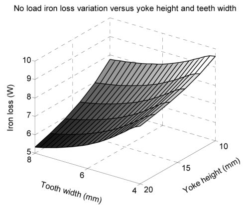
Fig. 22. Iron loss variations in terms of teeth width and yoke height at no-load conditions.
