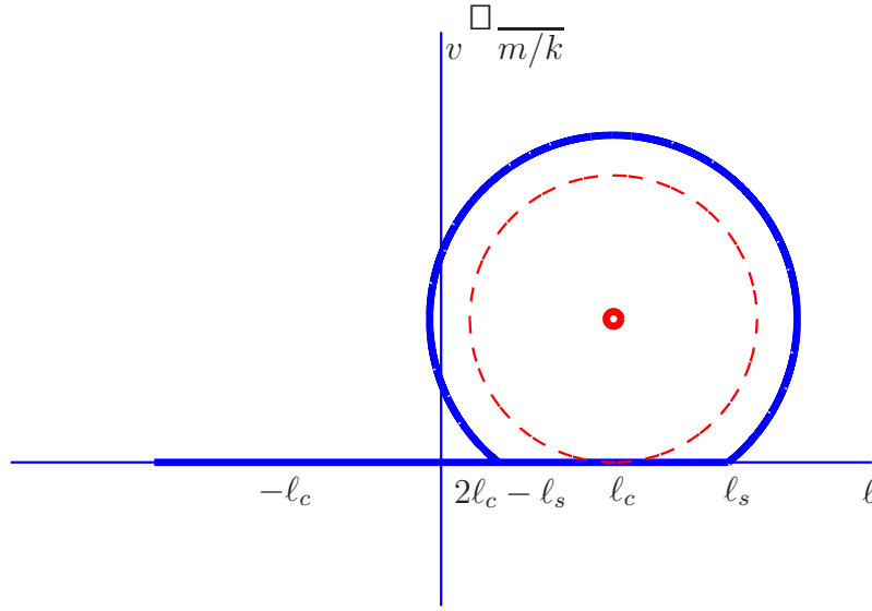
Figure 13. Phase plane for the hybrid model of stick-slip motion (see "Hybrid Model"). The sticking regime is the line 2\ell_c - \ell_s \leq \ell \leq \ell_s , and v = 0 . The slipping motion forms arcs of circles with center at (\ell_c, v_p \sqrt{m/k}) , for v > 0 . The center is marked with a circle. The dashed curve is a circle with center at (\ell_c, v_p \sqrt{m/k}) and radius v_p \sqrt{m/k} . All trajectories starting outside this circle converge to the limit cycle.
