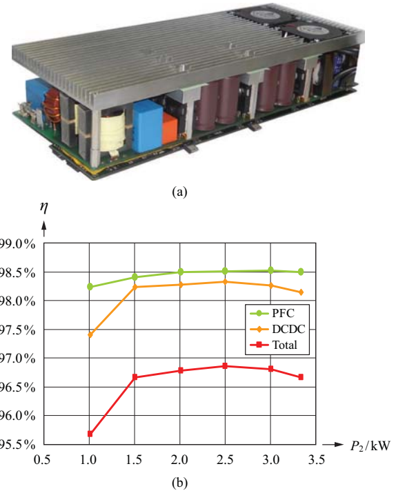
Fig. 32. 3.33 kW telecom power supply module (input stage: resonant transition mode boost-type PFC rectifier system with 3 phase-shifted branches, output stage: phase-shift full-bridge isolated DC/DC converter): (a) demonstrator of the system, power density: 2.5\text{ kW/dm}^3 , (b) efficiency curve.
