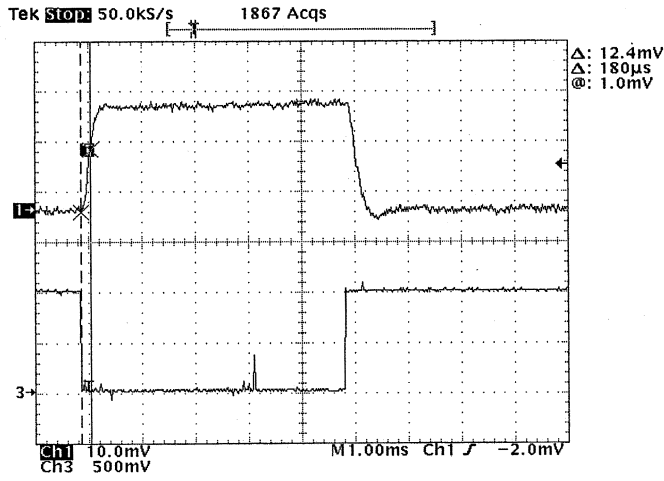
Fig. 13. Current step response at the aligned position (output current 10 mV = 1 A).
