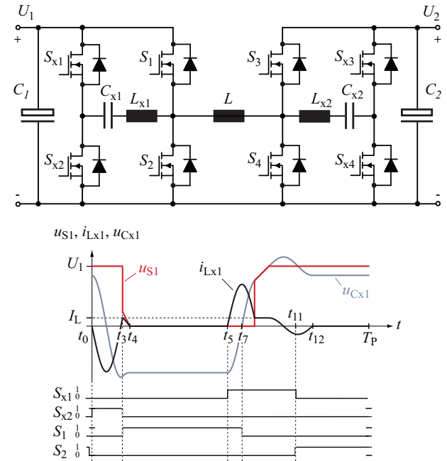
Fig. 4. ZCT-QZVT converter topology and typical waveforms for the buck operation mode.
