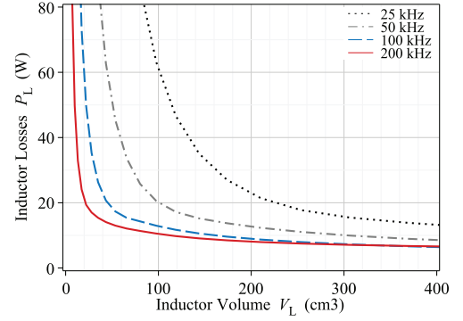
Fig. 12. CF-ZVS-M inductor losses in the worst-case operation point ( U_1 = 450V , U_2 = 225V , I_2 = I_{2,max} ) as a function of the inductor volume.
