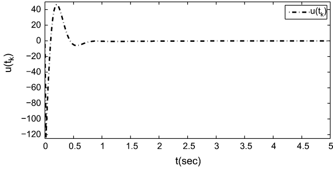
Fig. 5. Input of the inverted-pendulum model for sampling period is 0.02 s.
