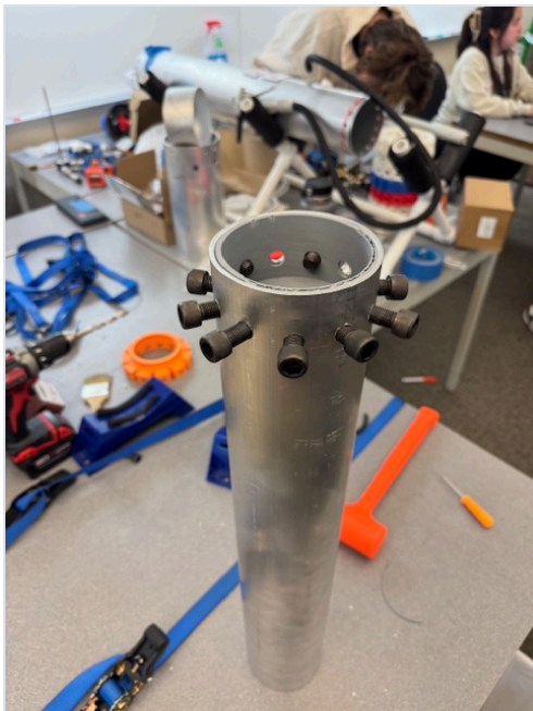
Figure 3. The assembled overwrapped test article.
