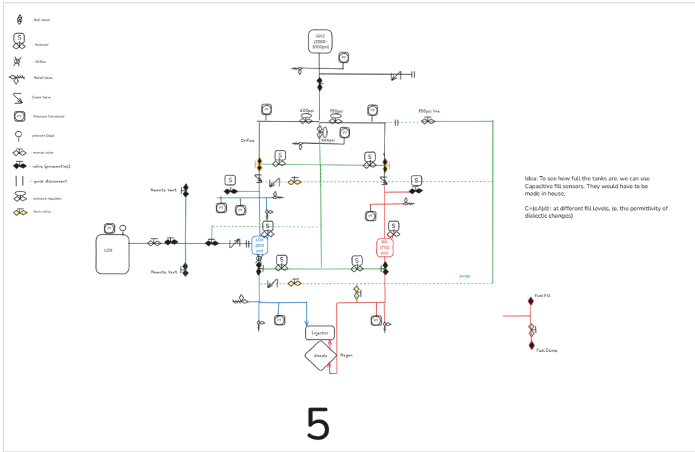
Figure 1. An early draft of the P&ID, iteration 5.
