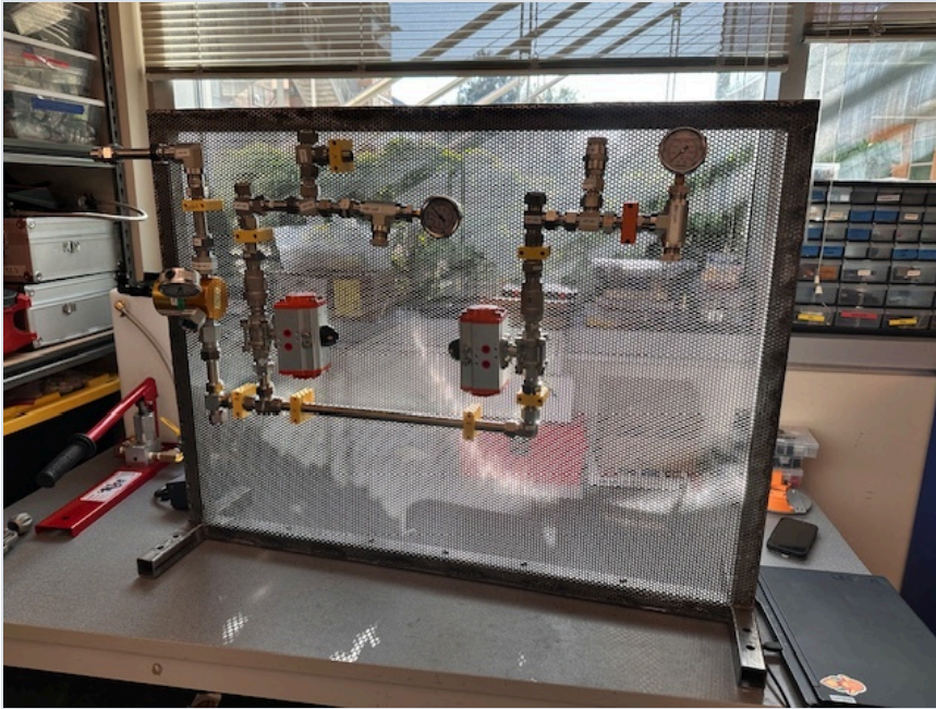
Figure 1. The completed LOX and ethanol fluid wall.
