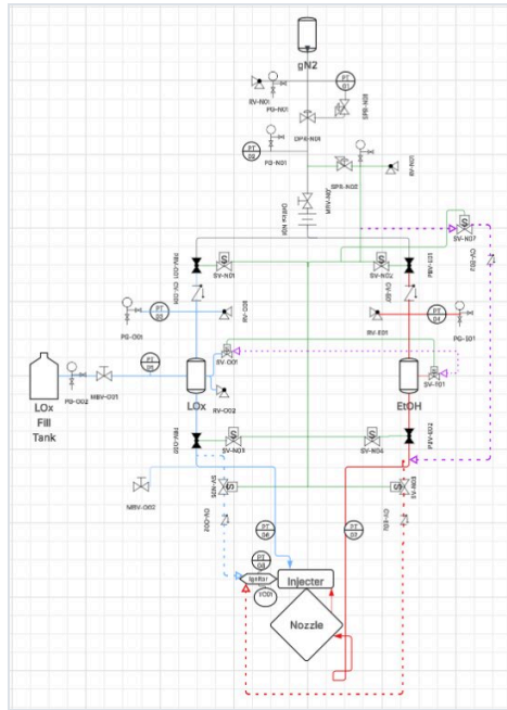
The LOX and ethanol P&ID, which I was mainly responsible for developing.
