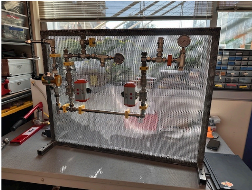
Figure 1. The completed LOX and ethanol fluid wall.
