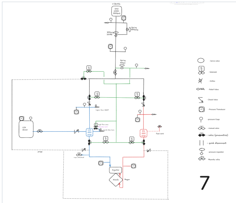
Figure 4. Iteration 7, as the architecture converged.
