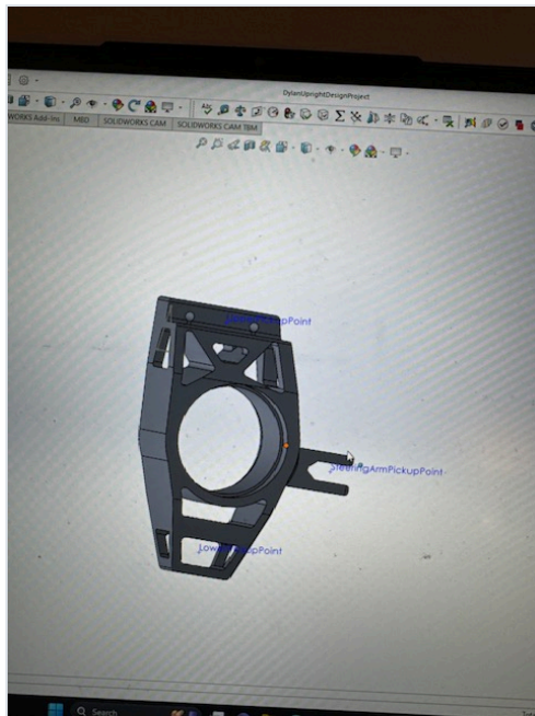
Figure 2. First iteration in SolidWorks.
