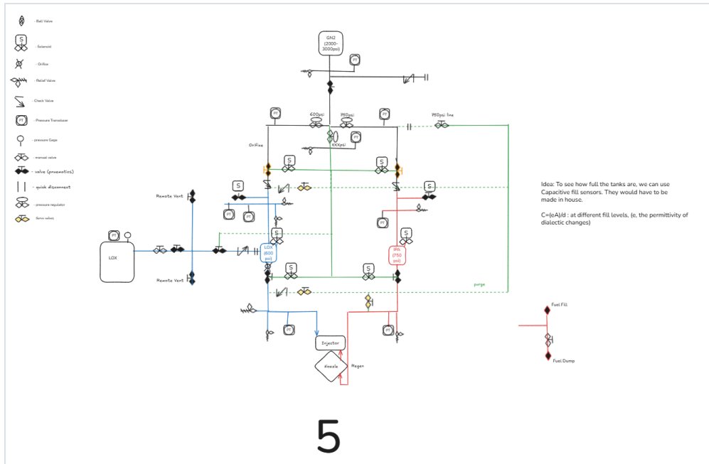
Figure 2. An early draft of the P&ID, iteration 5.
