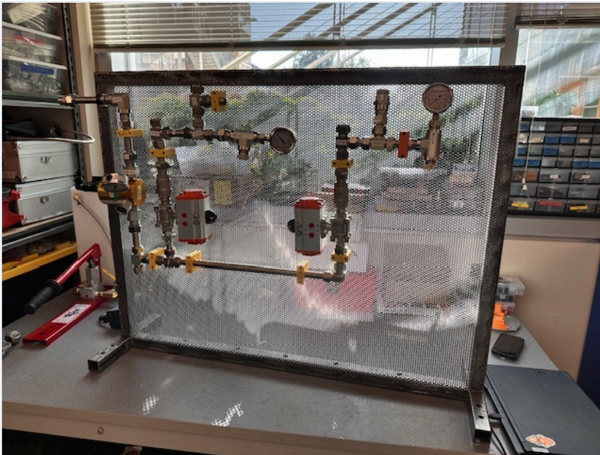
Figure 1. The LOX and ethanol fluid wall, partway through assembly.
