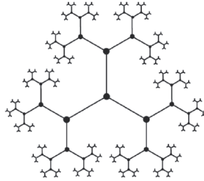
Figure 4: An infinite 3-regular tree you might have seen before in connection to SL_2(\mathbb{Q}_2) . Credit to Wikipedia.
