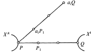
Figure 3: Diagram of the geodesics between the trees, from Serre's "Trees".
