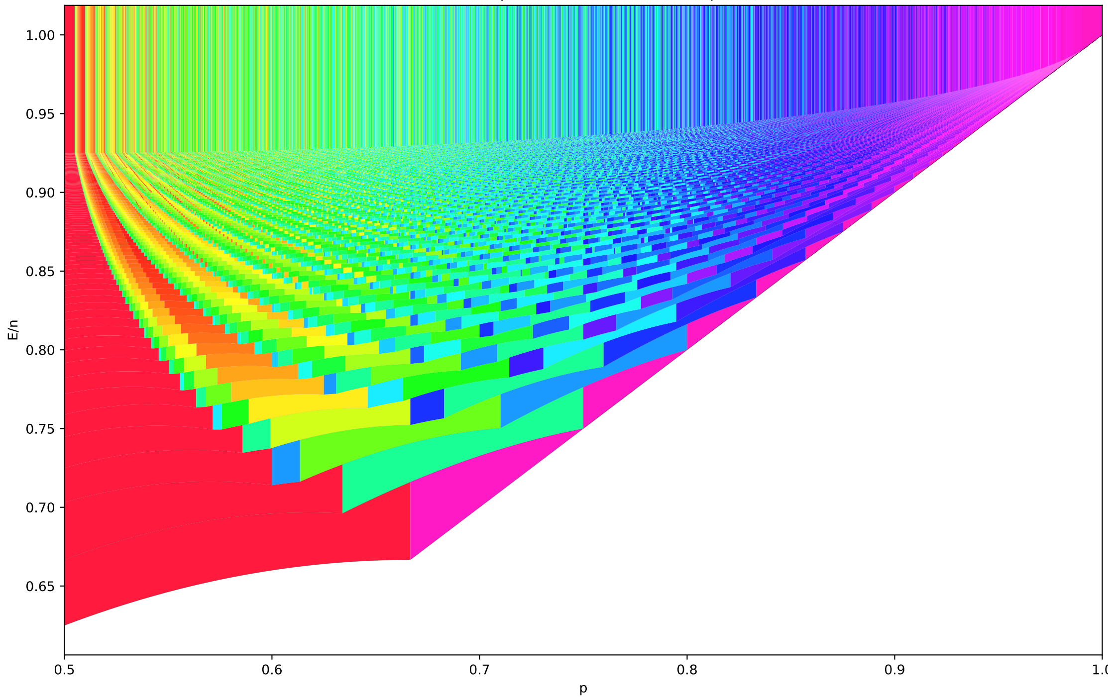
E[rank]/n vs p (n = 2-100, banded swap lines)
