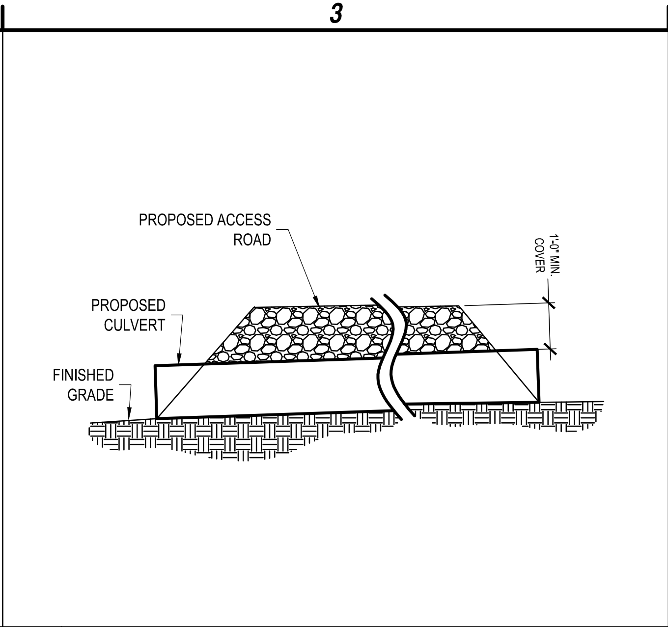
C3 TYPICAL CULVERT DETAIL SCALE: NOT TO SCALE
