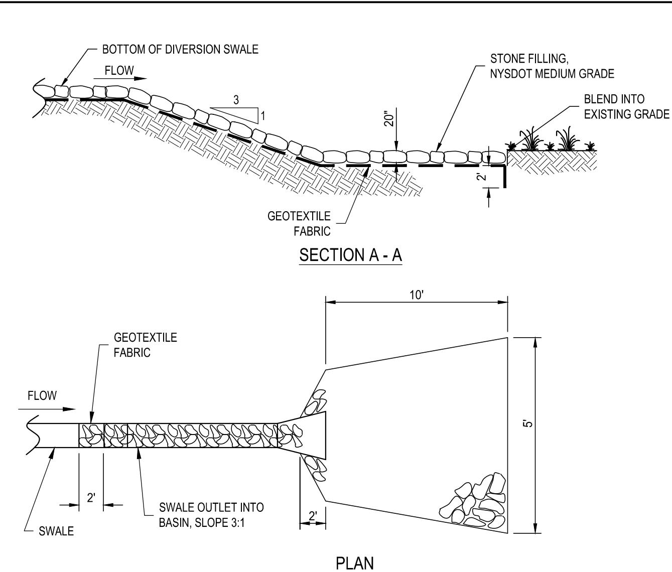
B2 ROCK OUTLET PROTECTION DETAIL SCALE: NOT TO SCALE
