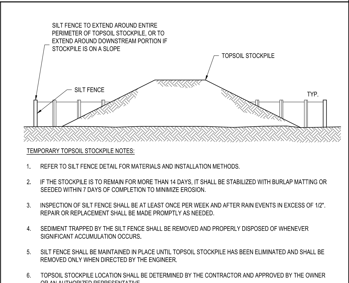
A4 TYPICAL TOPSOIL STOCKPILE DETAIL SCALE: NOT TO SCALE
