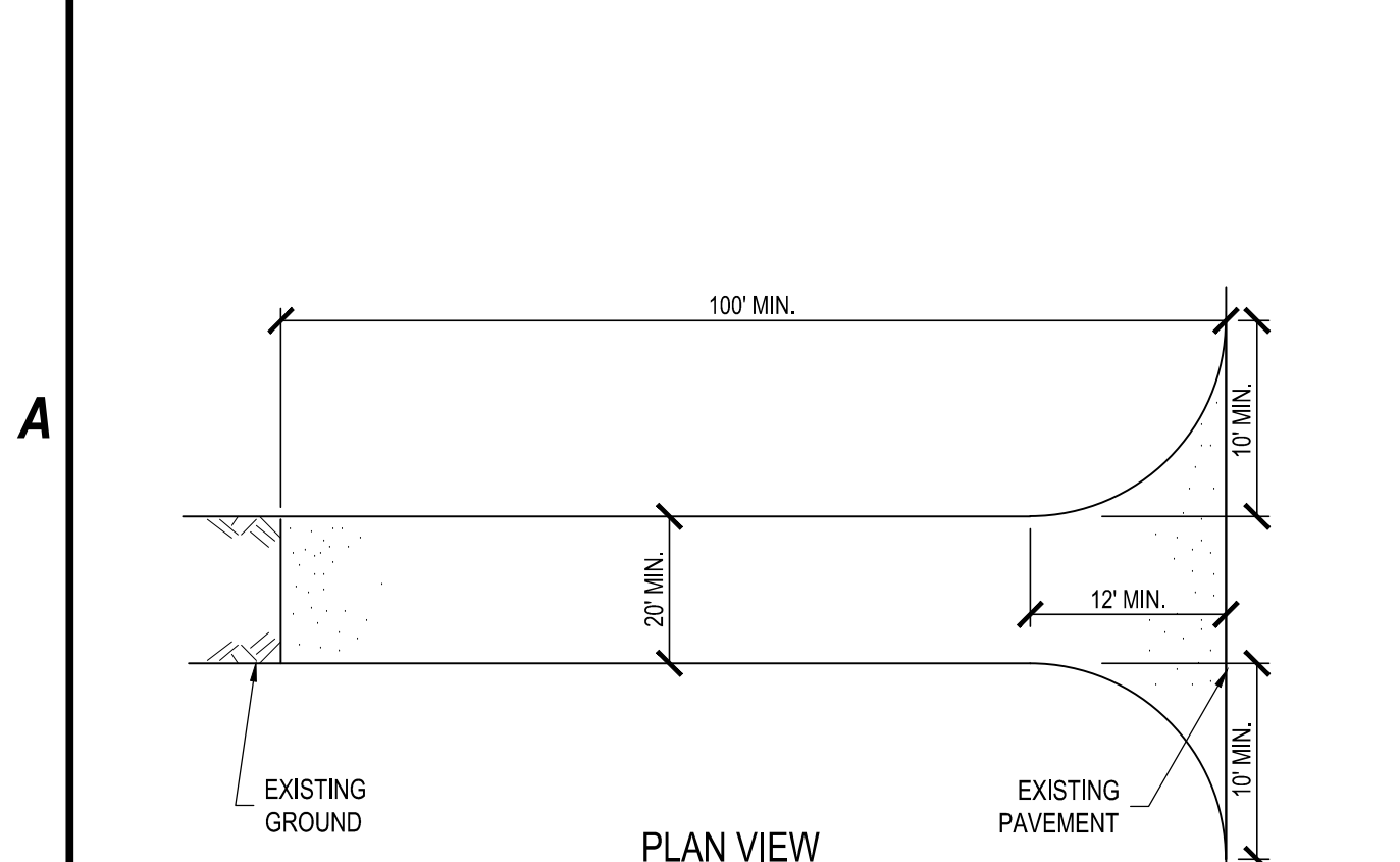
A1 STABILIZED CONSTRUCTION ENTRANCE DETAIL SCALE: NOT TO SCALE
