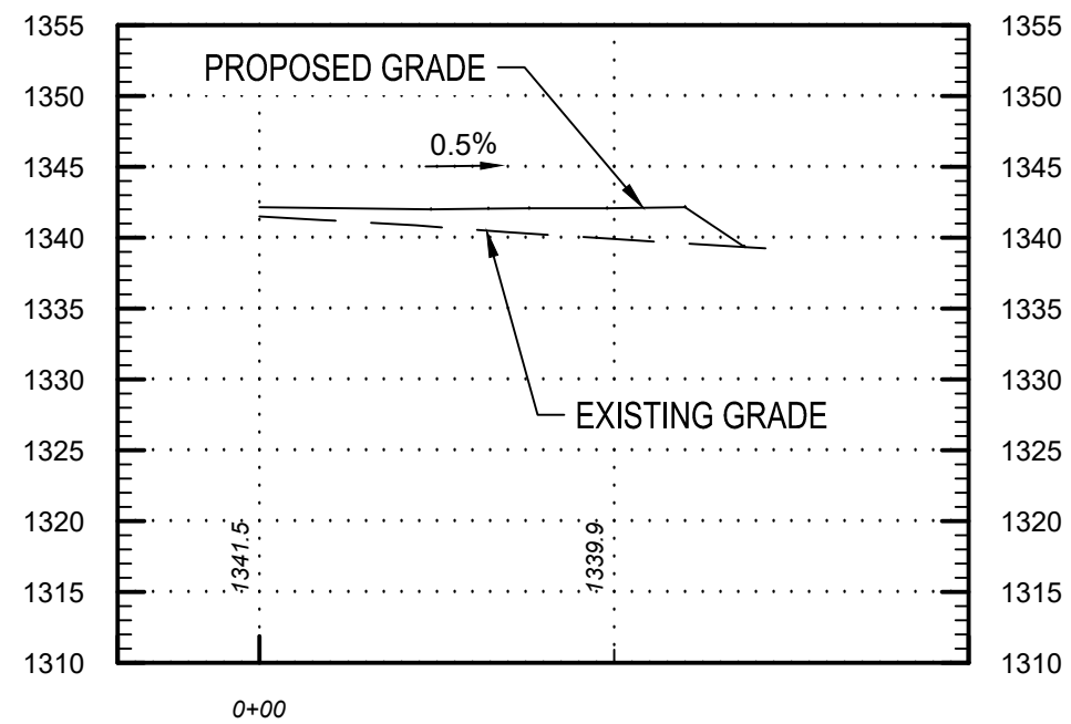
TURN ONE PROFILE
