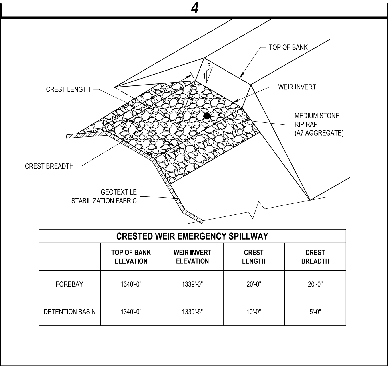
C4 CRESTED WEIR AND EMERGENCY SPILLWAY DETAIL SCALE: NOT TO SCALE
