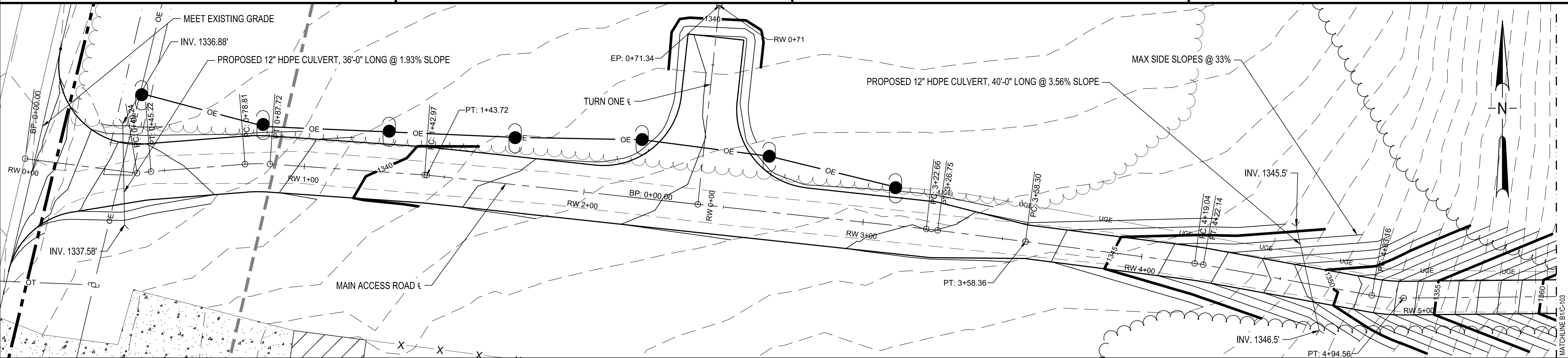
C1 MAIN ACCESS ROAD PLAN SCALE: 1" = 20'-0"
