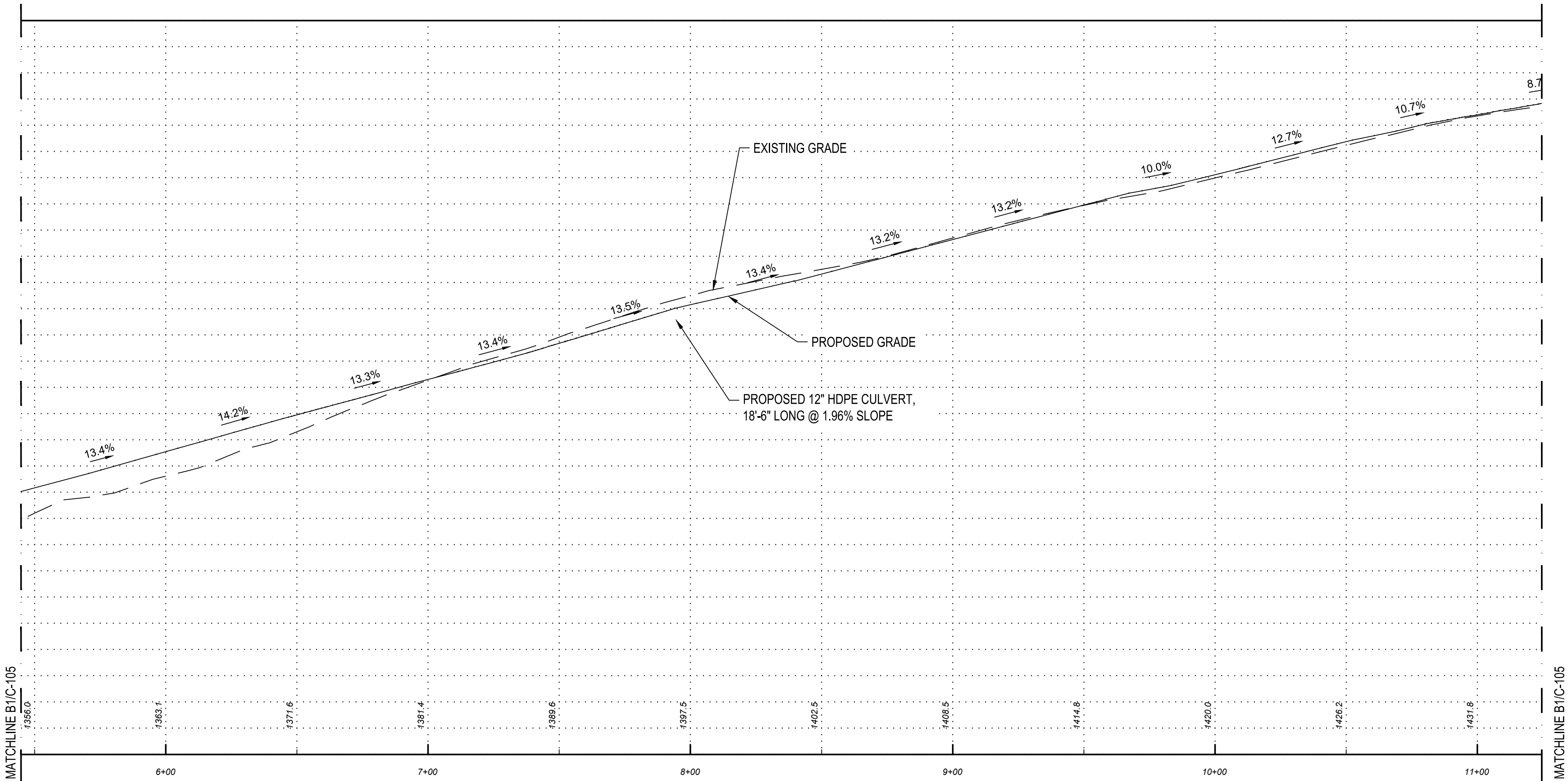
MAIN ACCESS ROAD PROFILE
