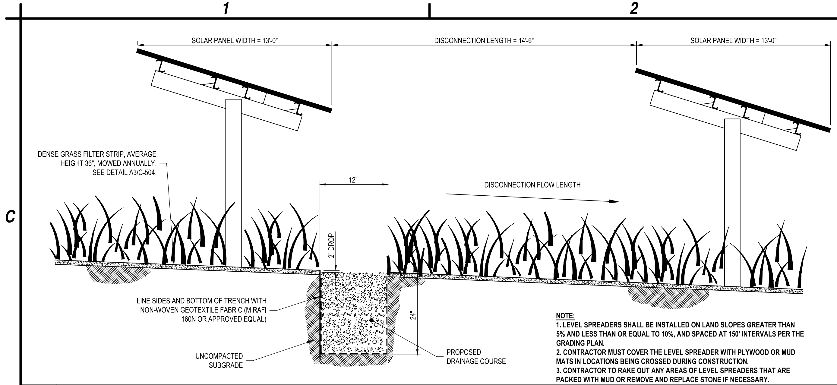
C1 LEVEL SPREADER TYPICAL DETAIL SCALE: NOT TO SCALE
