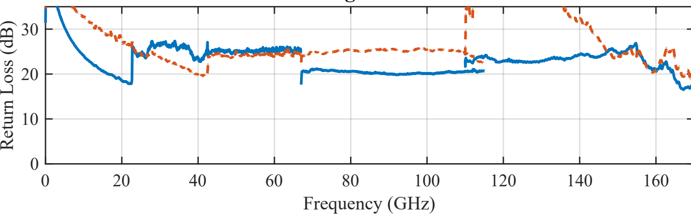
P1P4 Arc Return Loss
