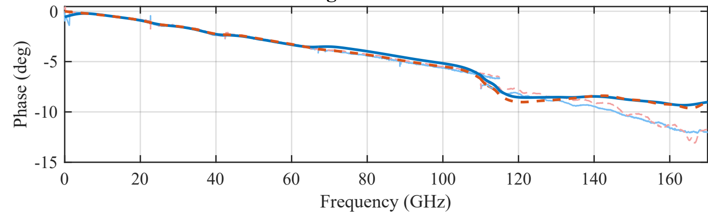
P3P4 Straight Transmission Phase
