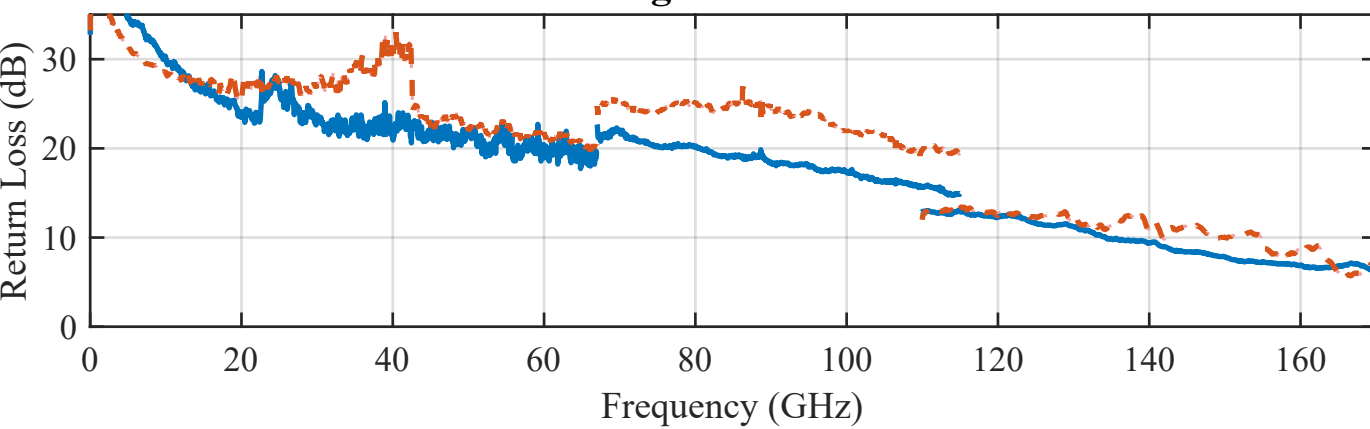
P1P4 Diagonal Return Loss
