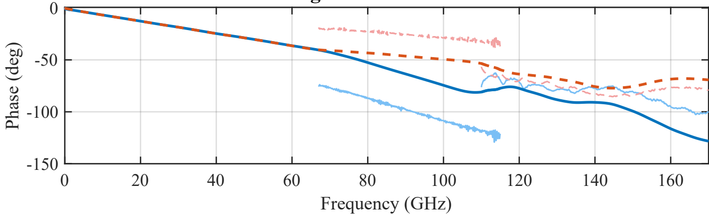
P1P4 Diagonal Transmission Phase
