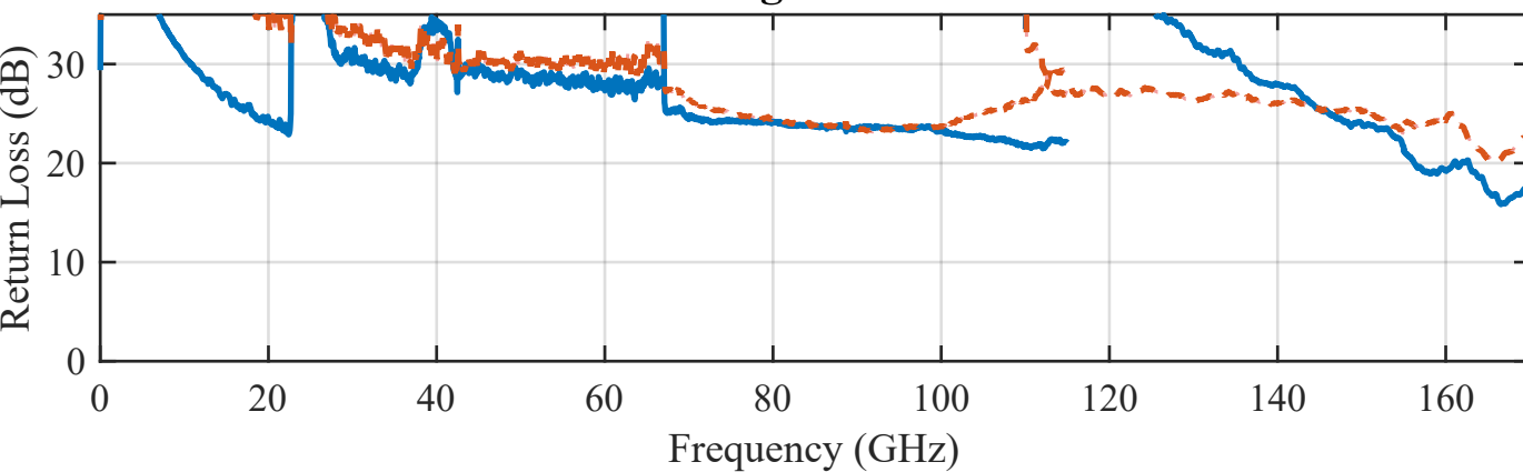
P3P4 Straight Return Loss
