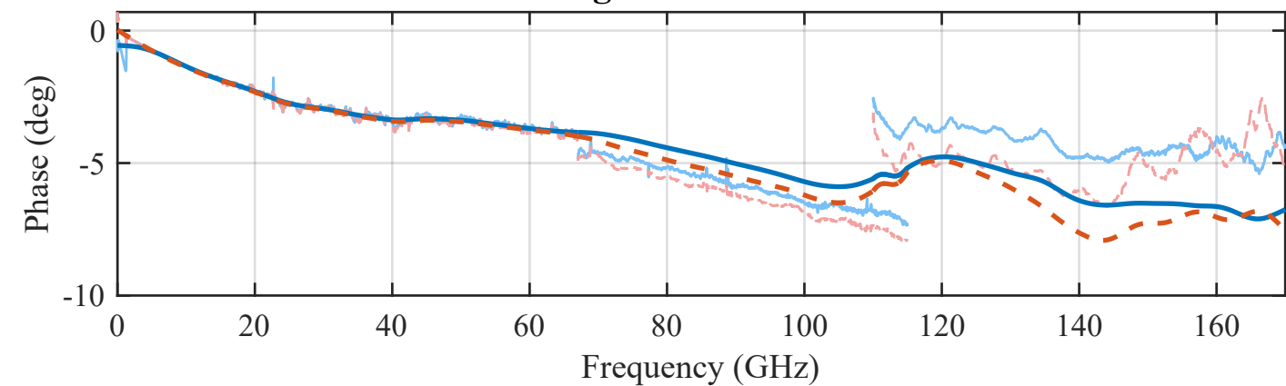
P1P4 Arc Transmission Phase
