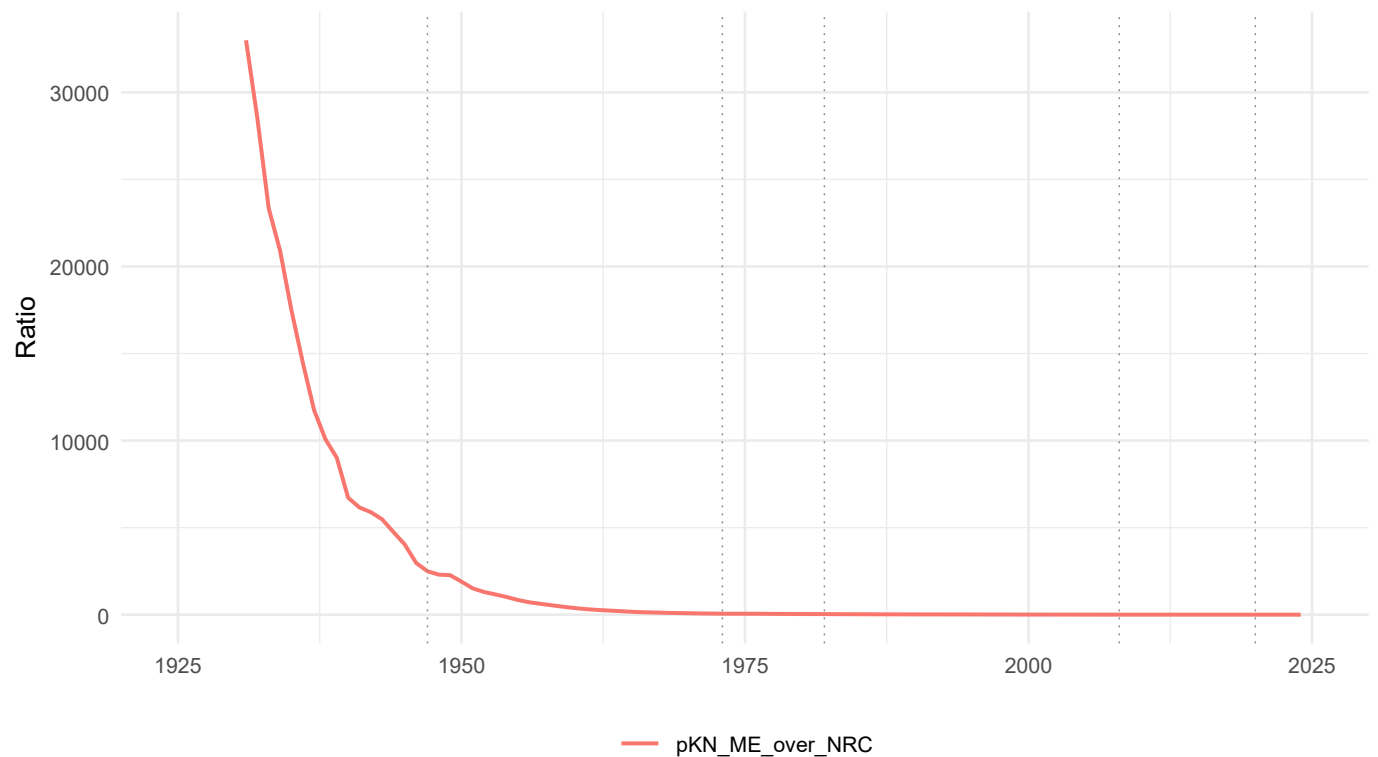
pKN ME/NRC ratio
