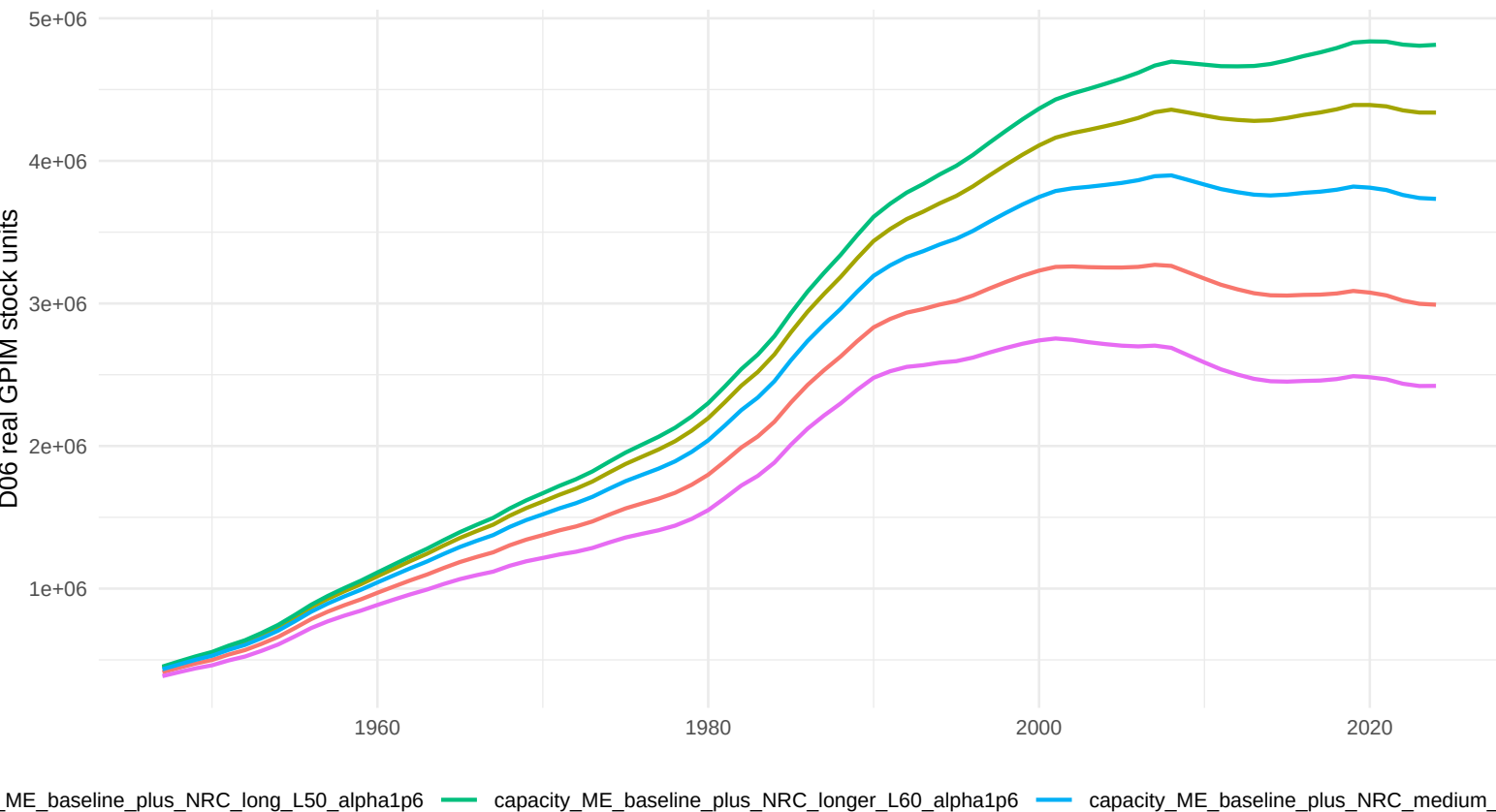
Real capacity under NRC service-life sensitivity
