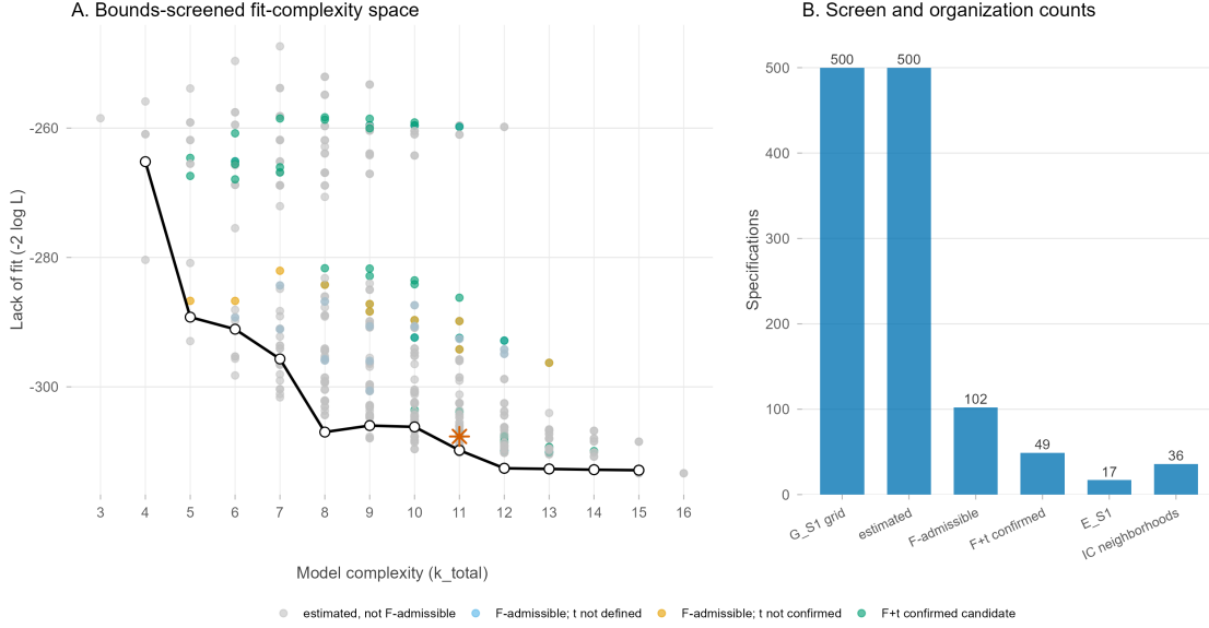
Figure 3: S1 Shrinking Specification Space
