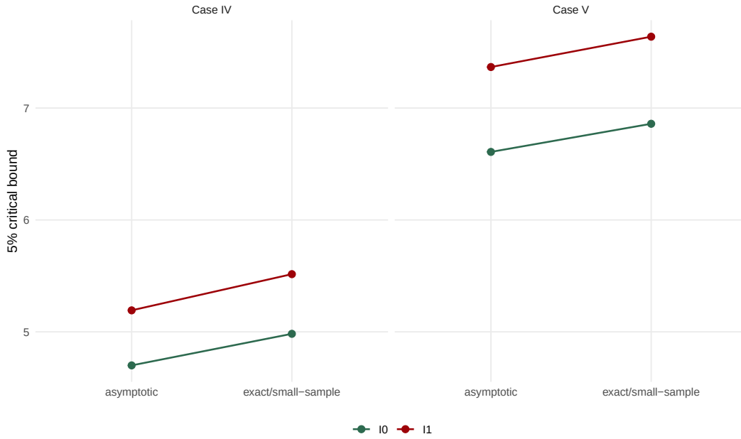
Figure 18: Exact-sample versus asymptotic critical bounds for Cases IV and V ( T = 65 ). Exact bounds computed via stochastic simulation (?).
