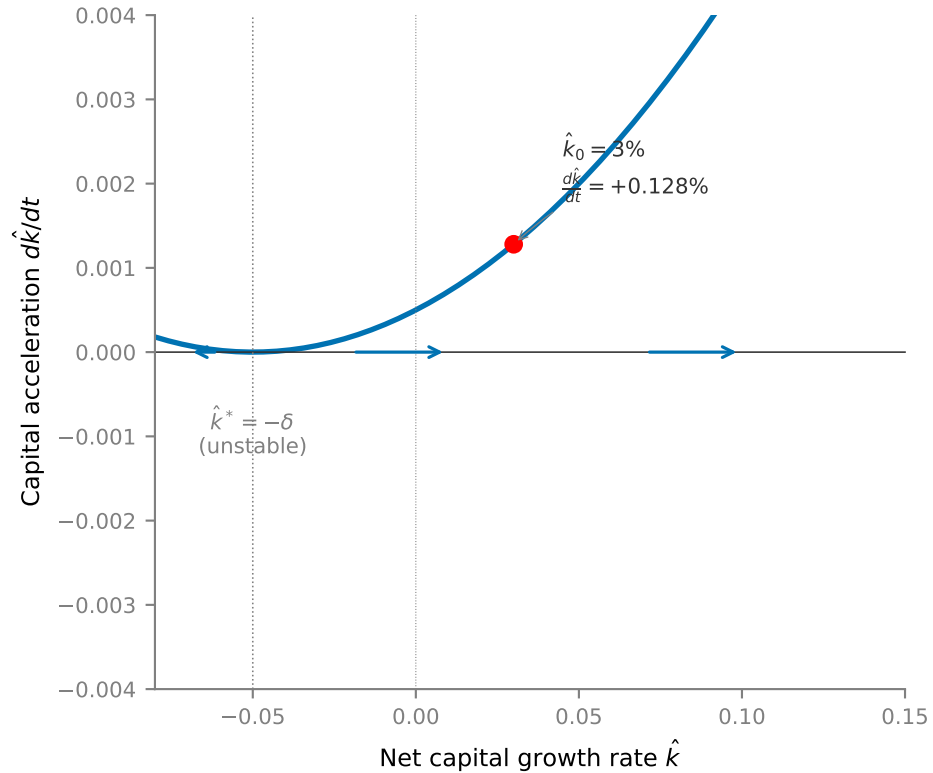
B. Explosive Growth Regime (Unstable)
