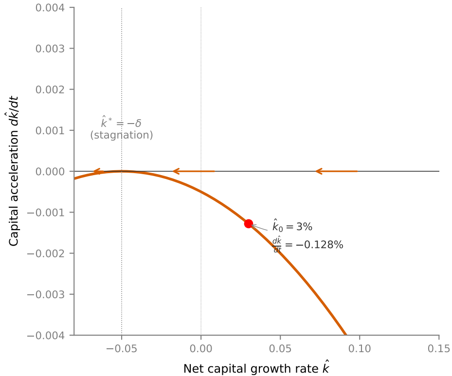
A. Overaccumulation Regime (Stable Stagnation)
