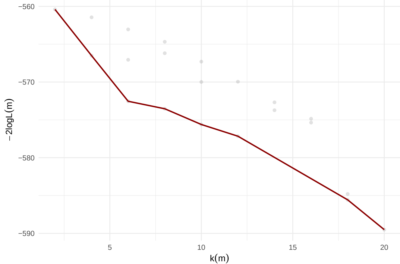
S2.1: VECM m=2 Admissible Cloud (fit-complexity)
