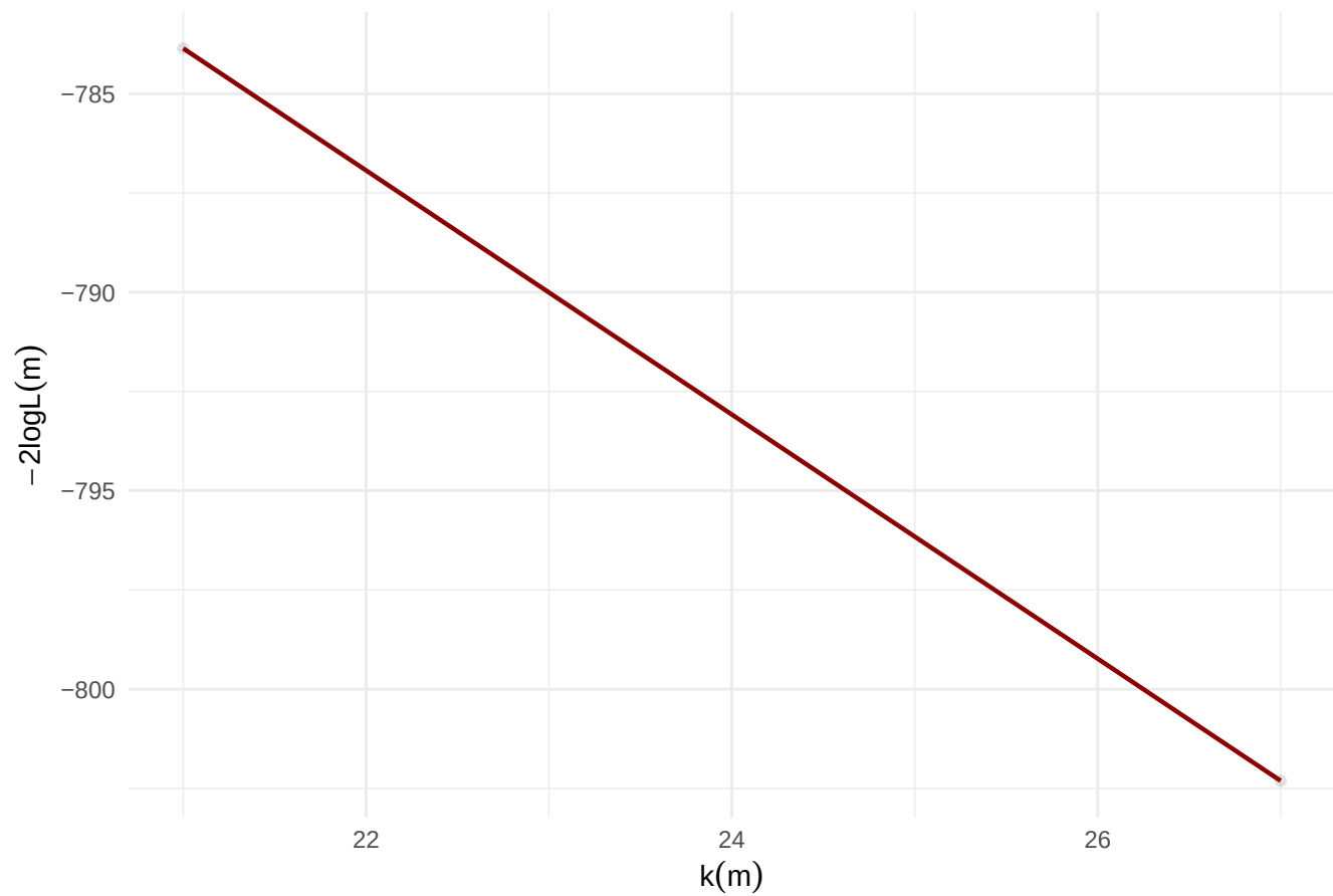
S2.1: VECM m=3 Admissible Cloud (fit-complexity)
