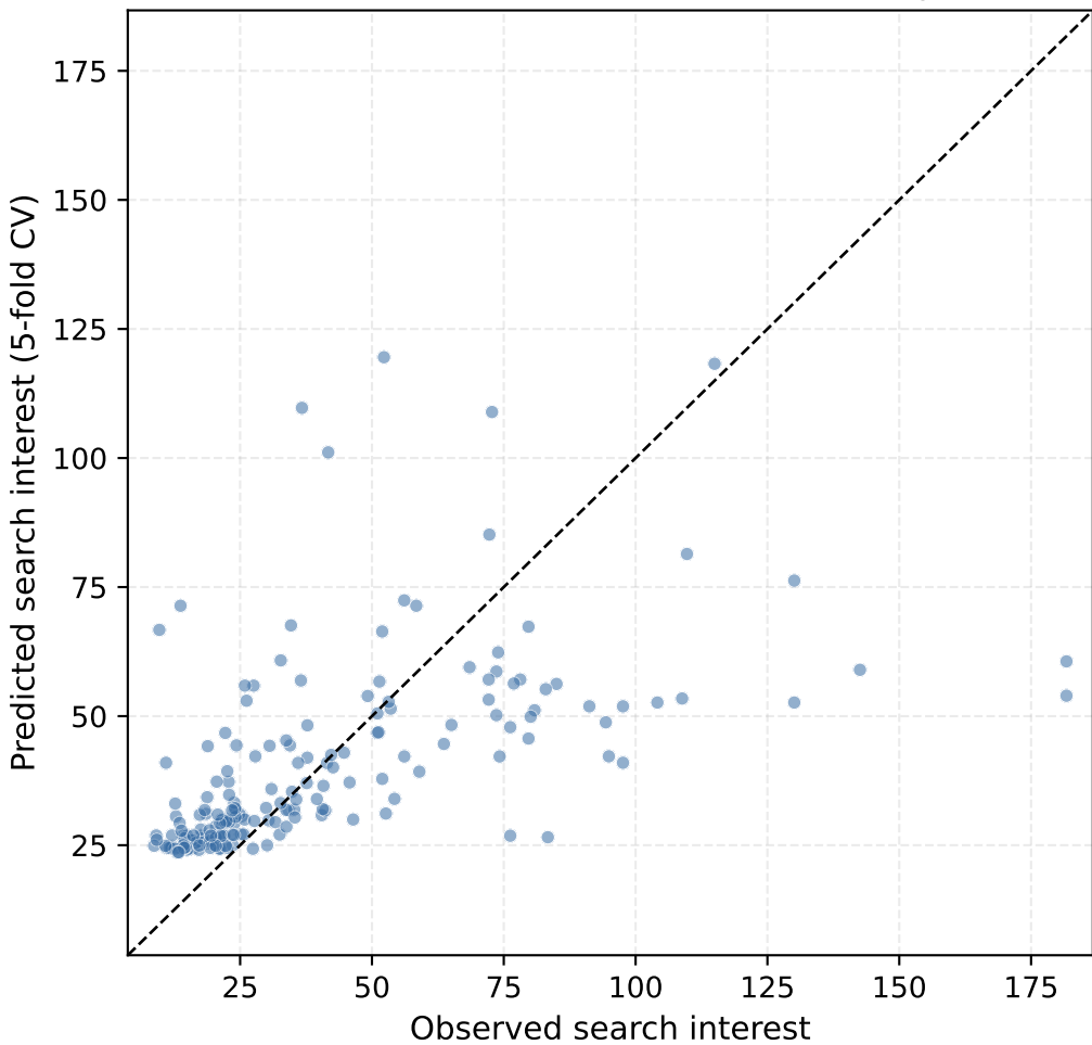
Gradient Boost: observed vs. cross-validated prediction
