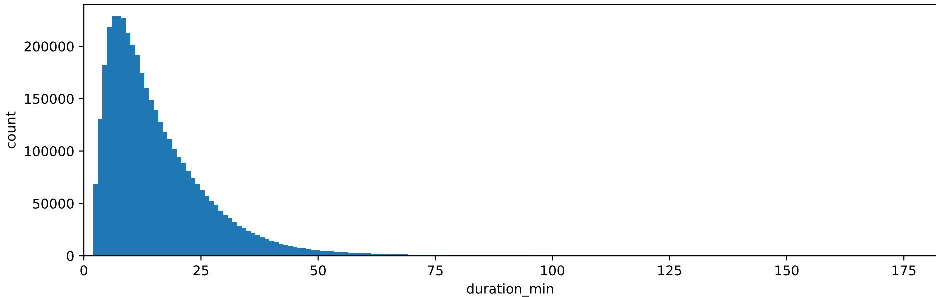
duration_min — after filter (n = 4,050,523)
